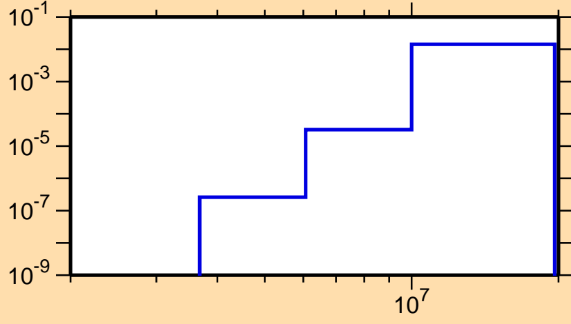
\sigma vs. E for ^{72}\text{Kr}(n,d)
