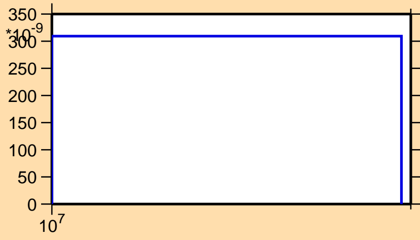
\sigma vs. E for ^{72}\text{Kr}(n,\text{pt})
