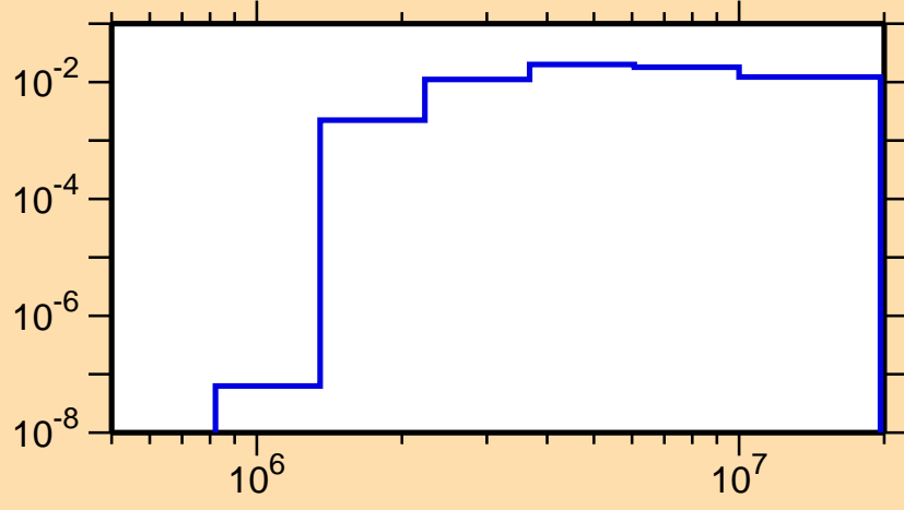
\sigma vs. E for ^{72}\text{Kr}(n,n_3)
