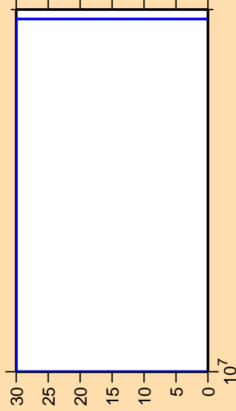
\Delta\sigma/\sigma vs. E for ^{72}\text{Kr} (mt 34)
