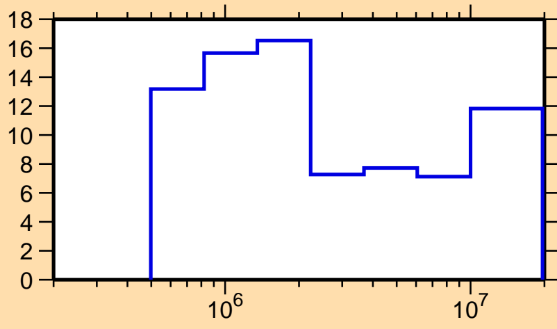
\Delta\sigma/\sigma vs. E for ^{72}\text{Kr}(n,\text{tot.})
