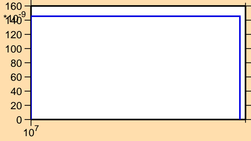
\sigma vs. E for ^{72}\text{Kr}(n,2n)
