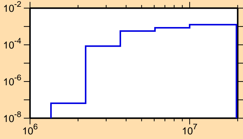
\sigma vs. E for ^{72}\text{Kr}(n,n\text{cont.})
