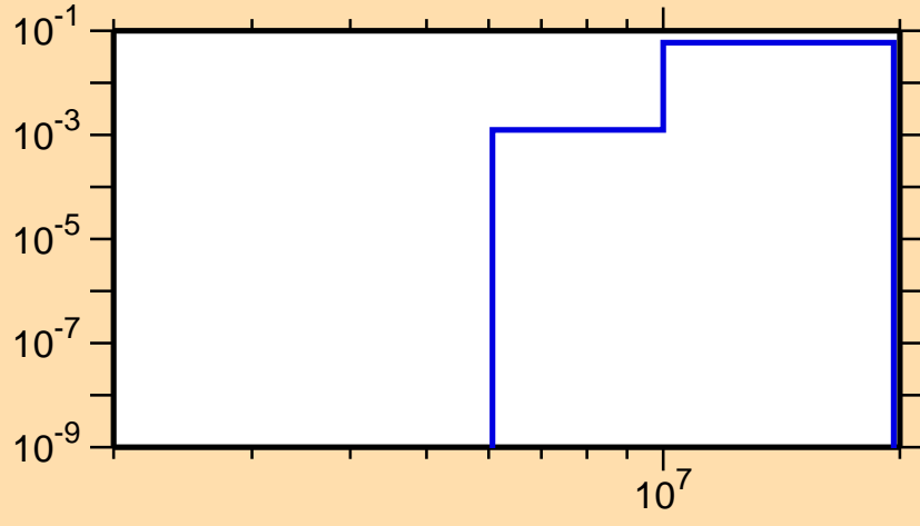
\sigma vs. E for ^{72}\text{Kr}(n,np)
