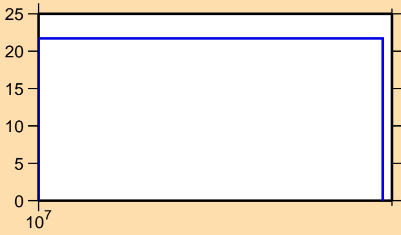
\Delta\sigma/\sigma vs. E for ^{72}\text{Kr}(n,\text{el.})
