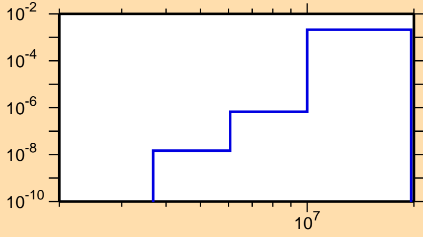
\sigma vs. E for ^{72}\text{Kr}(n,\text{He}3)
