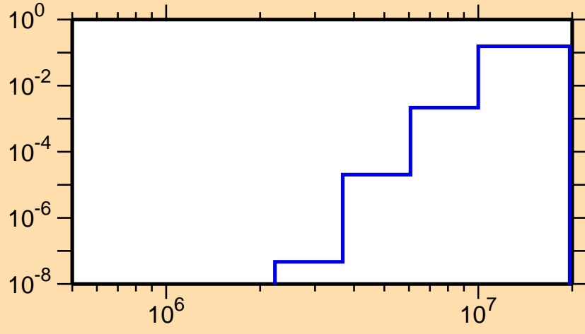
\sigma vs. E for ^{72}\text{Kr}(n,p\alpha)
