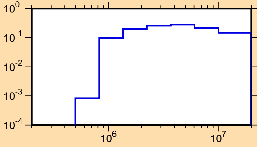
\sigma vs. E for ^{72}\text{Kr}(n,\text{inel.})
