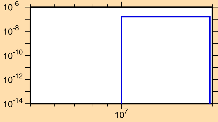
\sigma vs. E for ^{72}\text{Kr}(\text{mt } 45)
