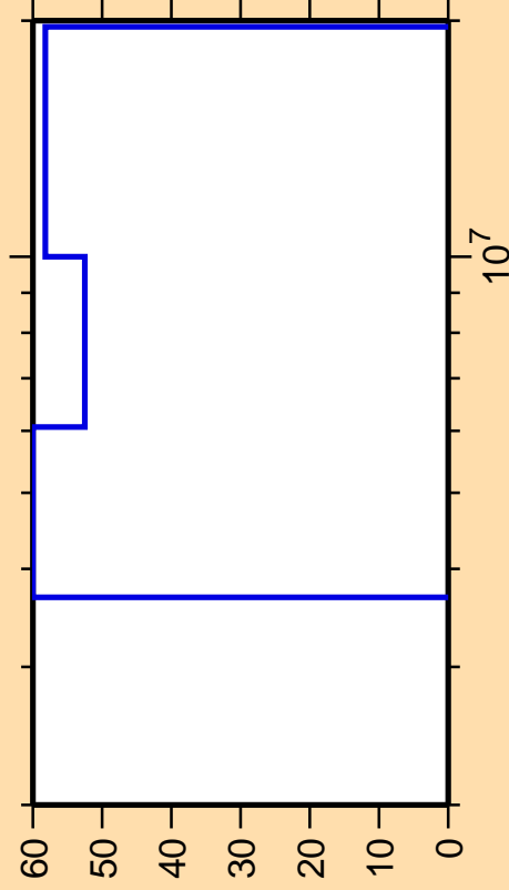
\Delta\sigma/\sigma vs. E for ^{72}\text{Kr}(n,np)
