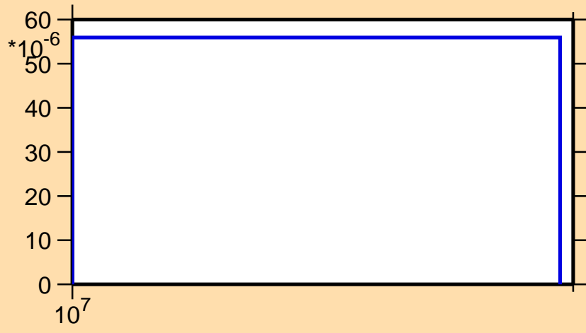
\sigma vs. E for ^{72}\text{Kr}(n,t)
