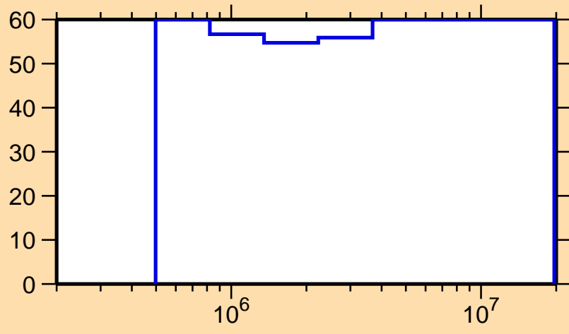
\Delta\sigma/\sigma vs. E for ^{72}\text{Kr}(n,\text{inel.})
