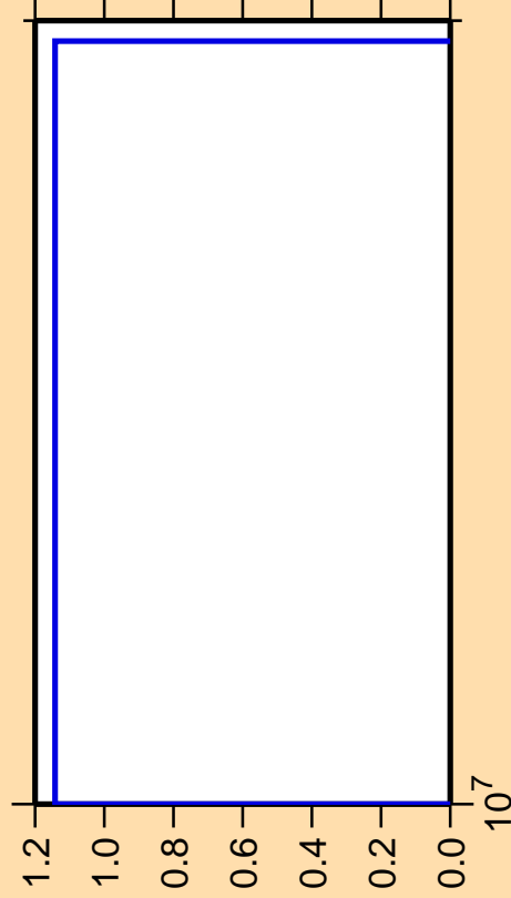
\Delta\sigma/\sigma vs. E for ^{72}\text{Kr}(n,nd)
