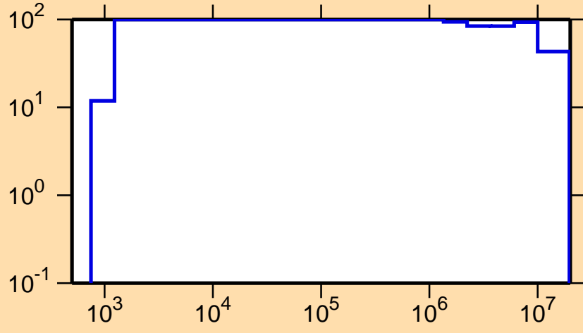
\Delta\sigma/\sigma vs. E for ^{72}\text{Kr}(n,\gamma)
