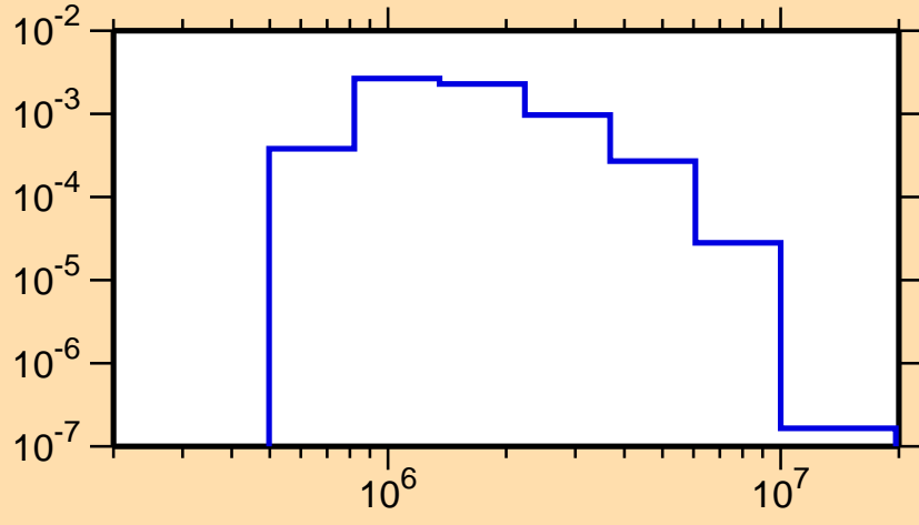
\sigma vs. E for ^{72}\text{Kr}(n,n_1)
