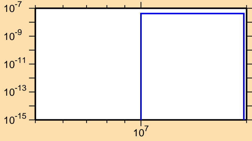
\sigma vs. E for ^{72}\text{Kr}(\text{mt117})
