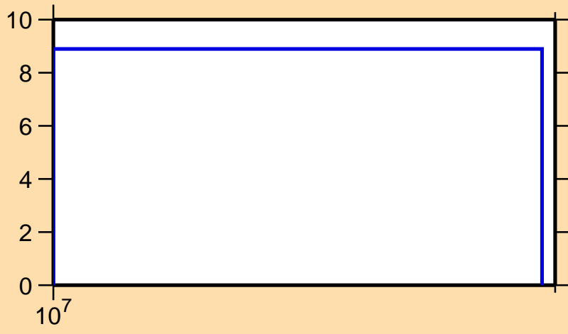
\Delta\sigma/\sigma vs. E for ^{72}\text{Kr}(n,\text{nonel.})
