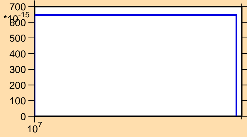
\sigma vs. E for ^{72}\text{Kr}(n,nd)
