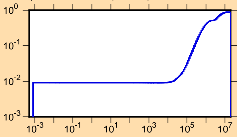
\mu vs. E for ^{74}\text{Kr}(\text{mt251})
