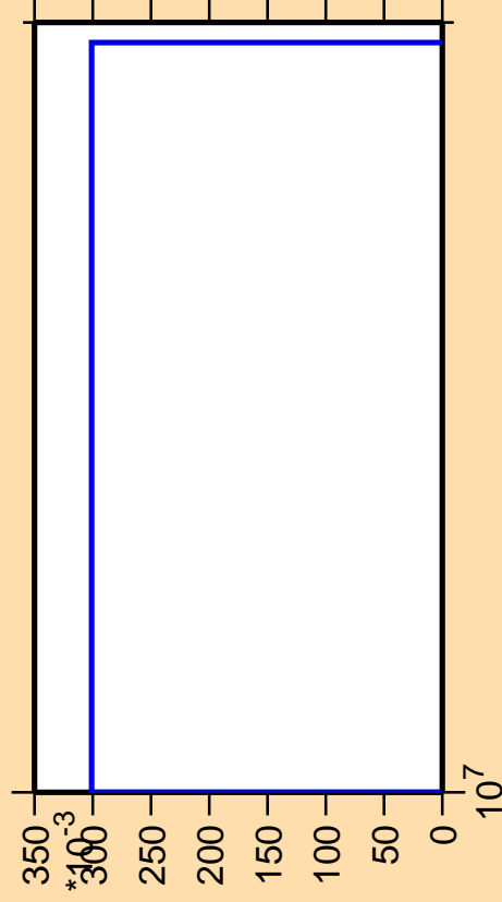
\Delta\sigma/\sigma vs. E for ^{74}\text{Kr} (mt 34)
