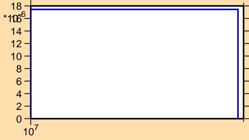
\sigma vs. E for ^{74}\text{Kr}(n,t)
