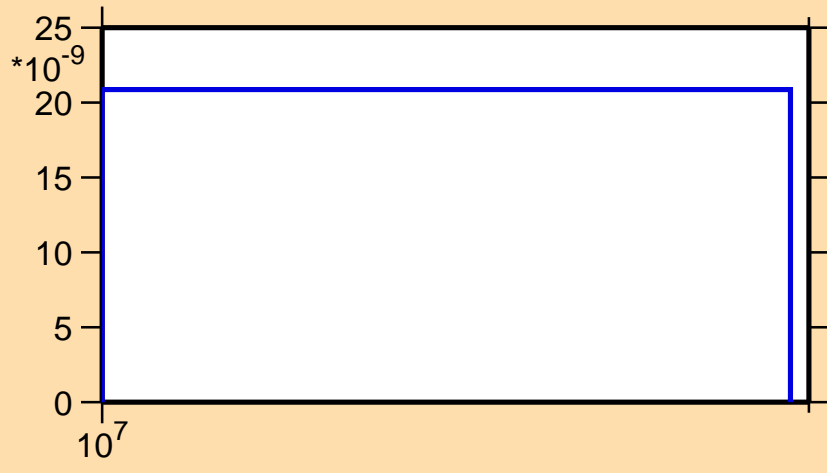
\sigma vs. E for ^{74}\text{Kr} (mt 45)
