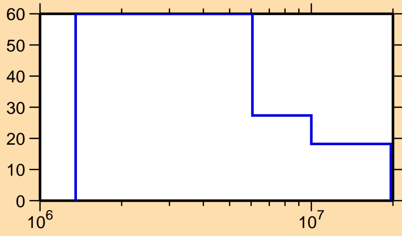
\Delta\sigma/\sigma vs. E for ^{74}\text{Kr}(n,ncont.)
