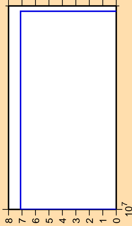
\Delta\sigma/\sigma vs. E for ^{74}\text{Kr}(n,\text{nd})
