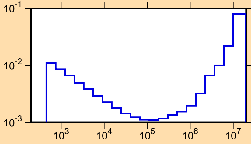
\sigma vs. E for ^{74}\text{Kr}(n,\alpha)
