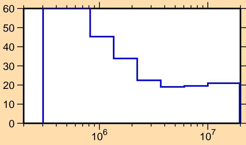
\Delta\sigma/\sigma vs. E for ^{74}\text{Kr}(n,n_1)
