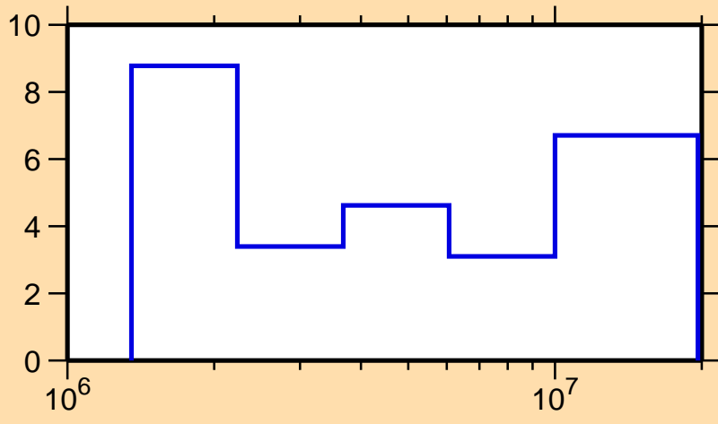
\Delta\sigma/\sigma vs. E for ^{74}\text{Kr}(n,el.)
