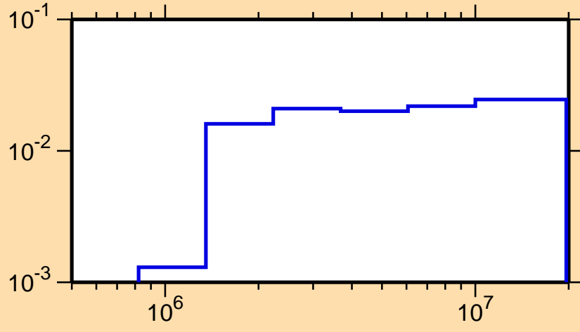
\sigma vs. E for ^{74}\text{Kr}(n,n_4)
