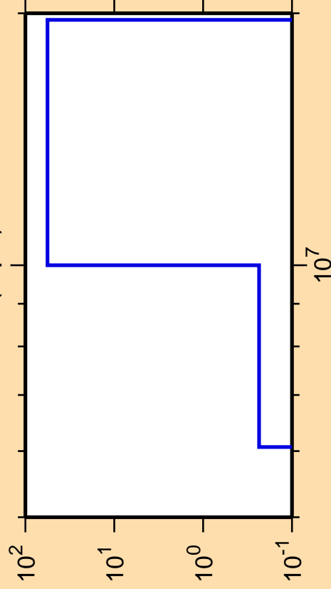
\Delta\sigma/\sigma vs. E for ^{74}\text{Kr}(n,pd)
