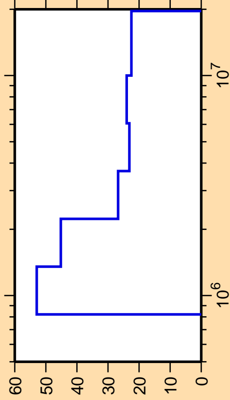
\Delta\sigma/\sigma vs. E for ^{74}\text{Kr}(n,n_4)
