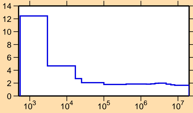
\sigma vs. E for ^{74}\text{Kr}(n,\text{nonel.})
