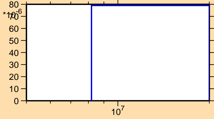
\sigma vs. E for ^{74}\text{Kr}(n,2n)
