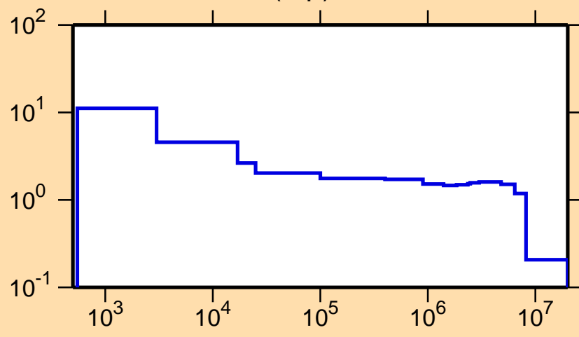
\sigma vs. E for ^{74}\text{Kr}(n,p)
