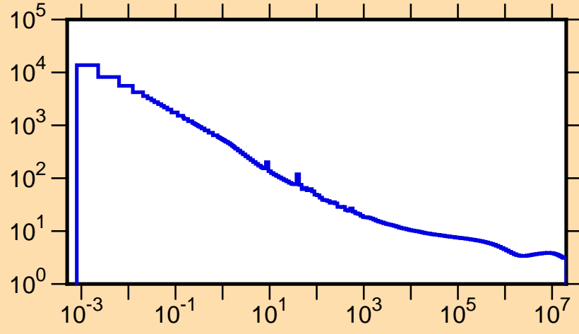
\sigma vs. E for ^{75}\text{Kr}(n,\text{tot.})
