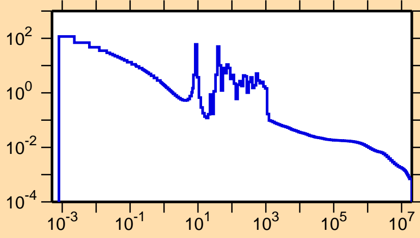
\sigma vs. E for ^{75}\text{Kr}(n,\gamma)
