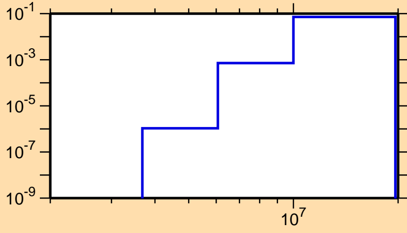
\sigma vs. E for ^{75}\text{Kr}(n,p\alpha)
