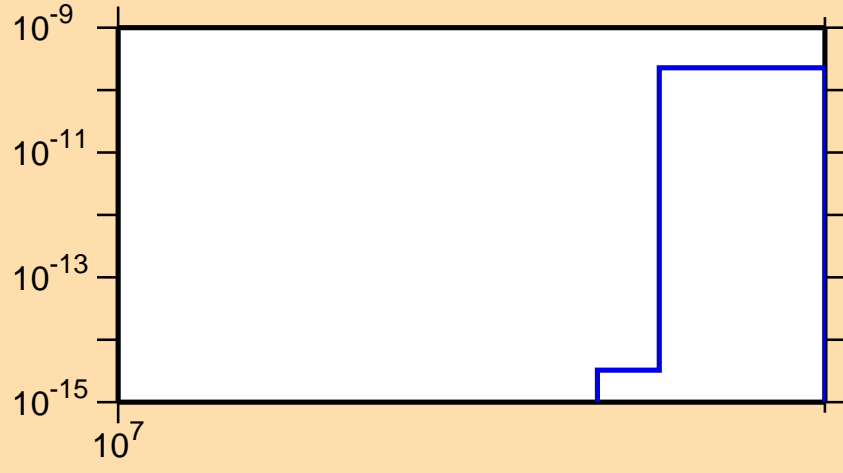
\sigma vs. E for ^{76}\text{Kr}(n,\text{pt})
