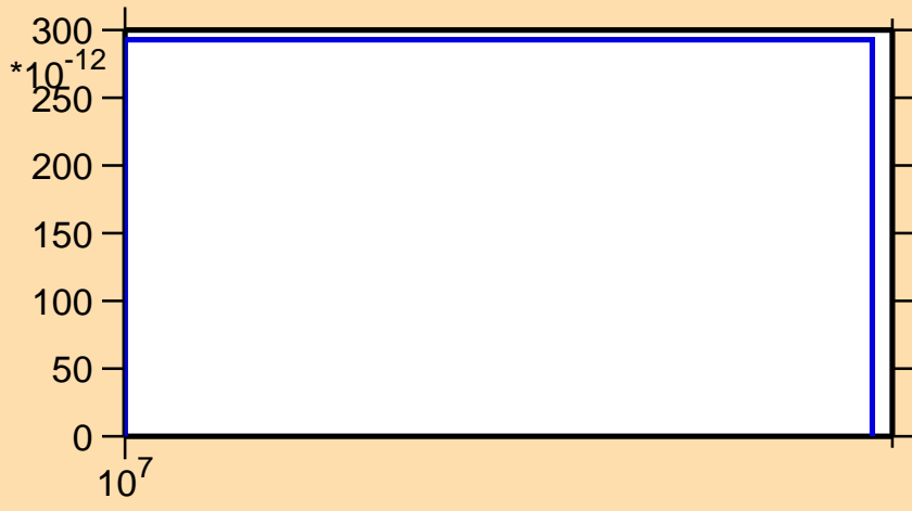
\sigma vs. E for ^{76}\text{Kr} (mt 45)
