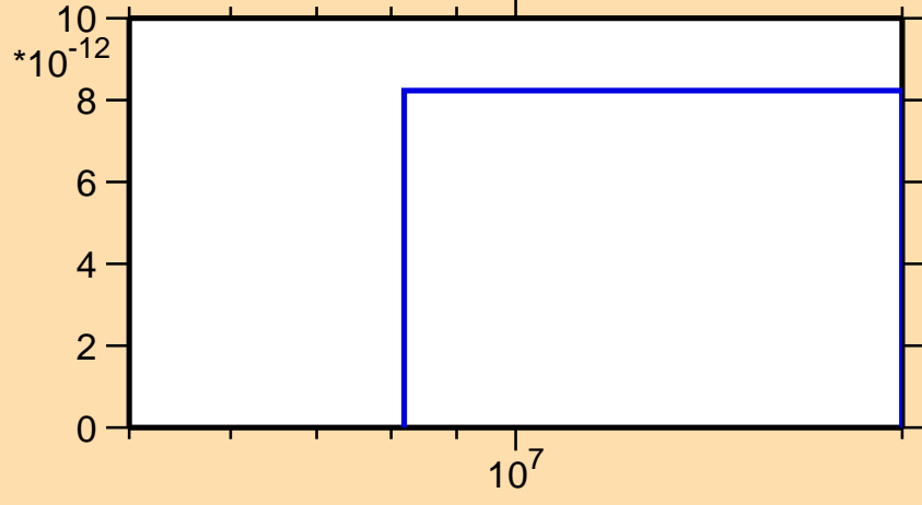
\sigma vs. E for ^{76}\text{Kr}(n,nd)
