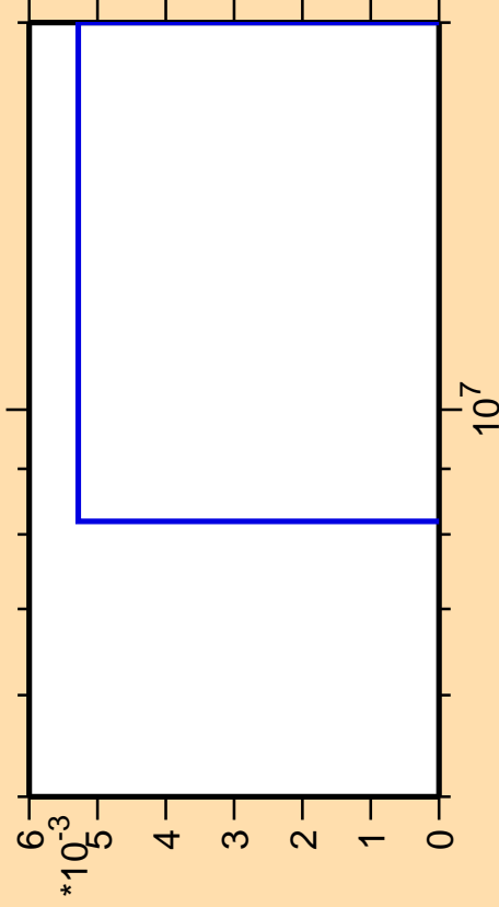
\Delta\sigma/\sigma vs. E for ^{76}\text{Kr}(\text{mt } 34)
