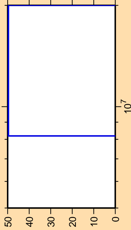
\Delta\sigma/\sigma vs. E for ^{76}\text{Kr}(n,nd)
