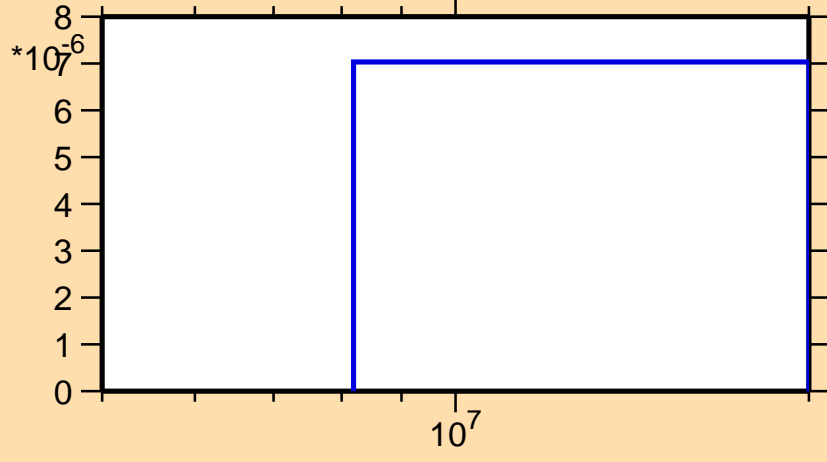
\sigma vs. E for ^{76}\text{Kr}(n,\text{pd})
