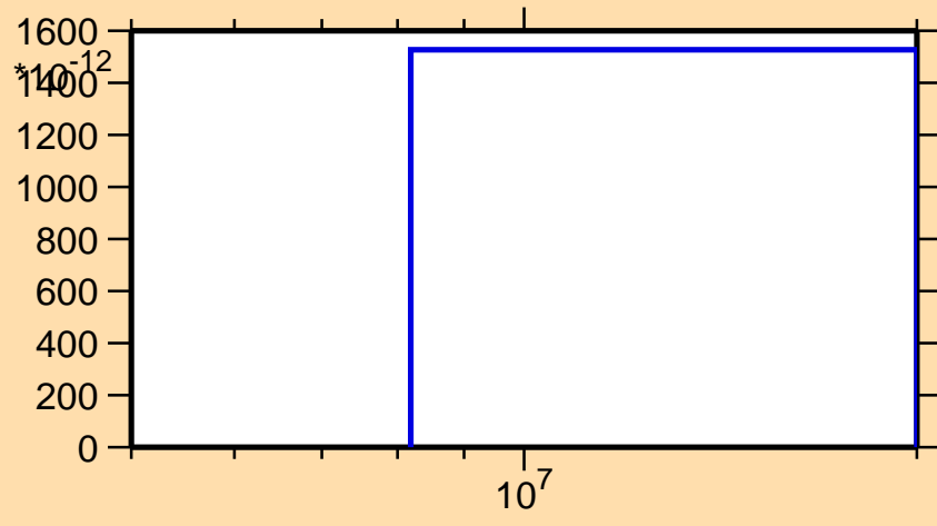
\sigma vs. E for ^{77}\text{Kr}(n,2n\alpha)
