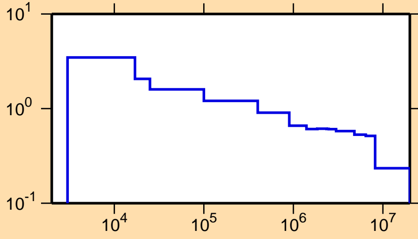
\sigma vs. E for ^{77}\text{Kr}(n,p)
