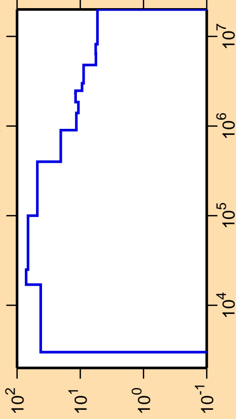
\Delta\sigma/\sigma vs. E for ^{77}\text{Kr}(n,\text{nonel.})
