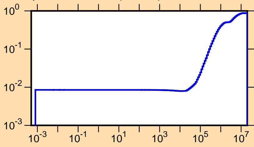
\mu vs. E for ^{79}\text{Kr}(\text{mt251})
