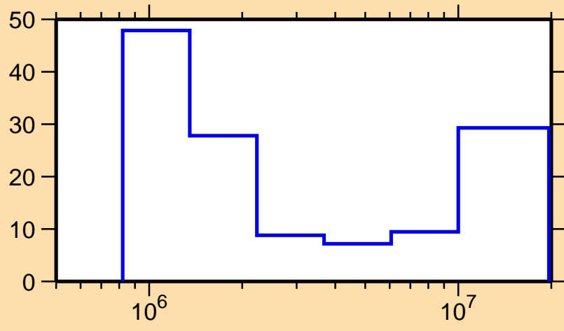
\Delta\sigma/\sigma vs. E for ^{79}\text{Kr}(n,ncont.)
