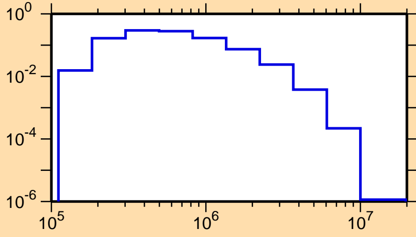
\sigma vs. E for ^{79}\text{Kr}(n,n_2)
