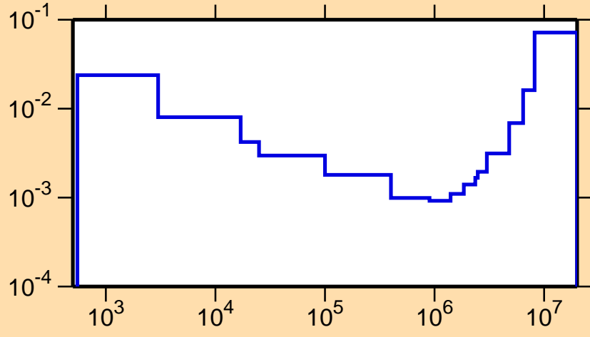
\sigma vs. E for ^{79}\text{Kr}(n,\alpha)
