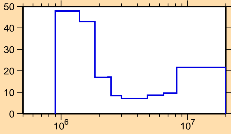
\Delta\sigma/\sigma vs. E for ^{79}\text{Kr}(n,n\text{cont.})
