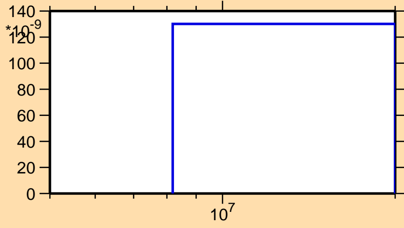
\sigma vs. E for ^{79}\text{Kr}(n,nd)
