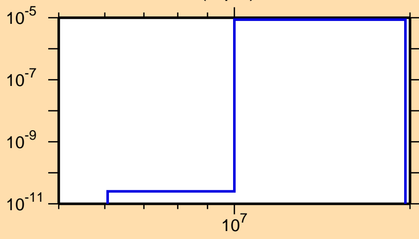
\sigma vs. E for ^{79}\text{Kr}(n,p\alpha)
