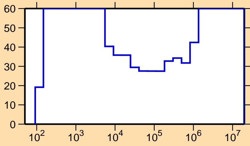
\Delta\sigma/\sigma vs. E for ^{79}\text{Kr}(n,\gamma)
