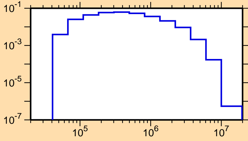
\sigma vs. E for ^{79}\text{Kr}(n,n_4)
