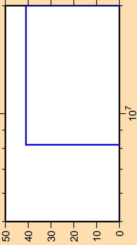
\Delta\sigma/\sigma vs. E for ^{79}\text{Kr}(n,2n)
