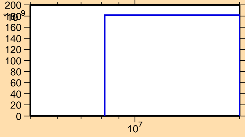
\sigma vs. E for ^{79}\text{Kr}(n,2np)
