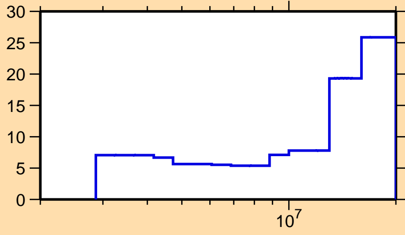
\Delta\sigma/\sigma vs. E for ^{80}\text{Kr}(n,inel.)
