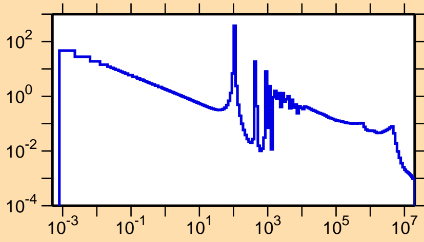
\sigma vs. E for ^{80}\text{Kr}(n,\gamma)
