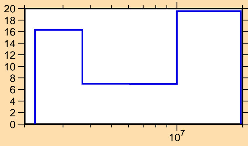
\Delta\sigma/\sigma vs. E for ^{80}\text{Kr}(n,n\text{cont.})
