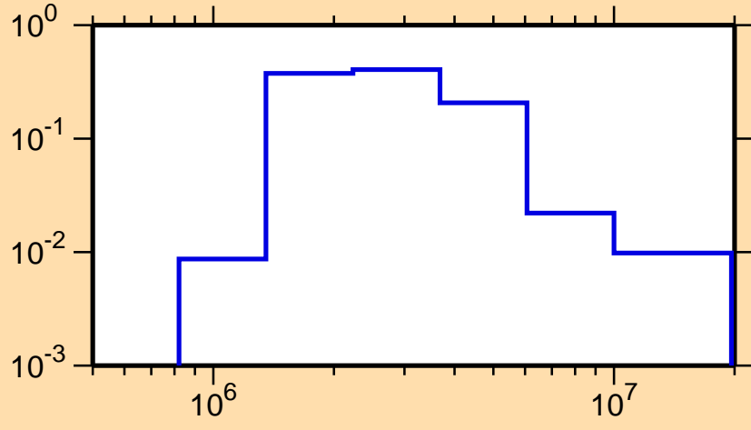
\sigma vs. E for ^{80}\text{Kr}(n,n_2)
