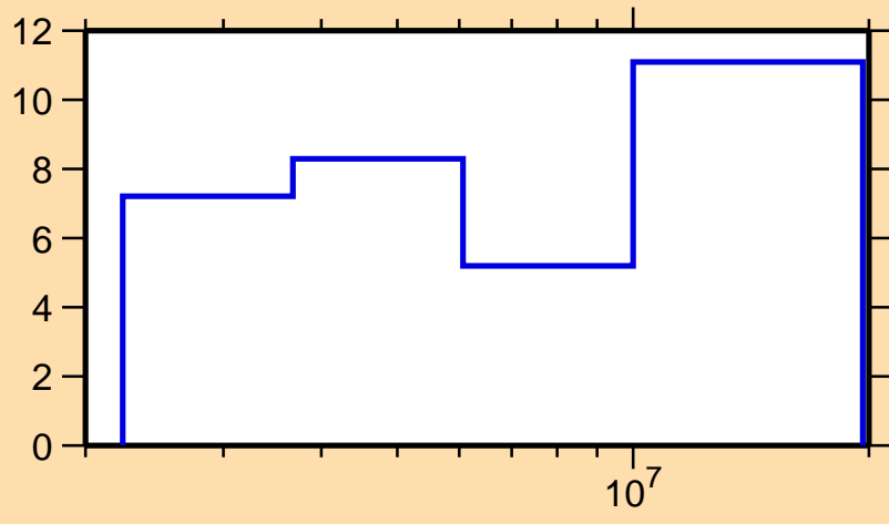
\Delta\sigma/\sigma vs. E for ^{80}\text{Kr}(n,el.)
