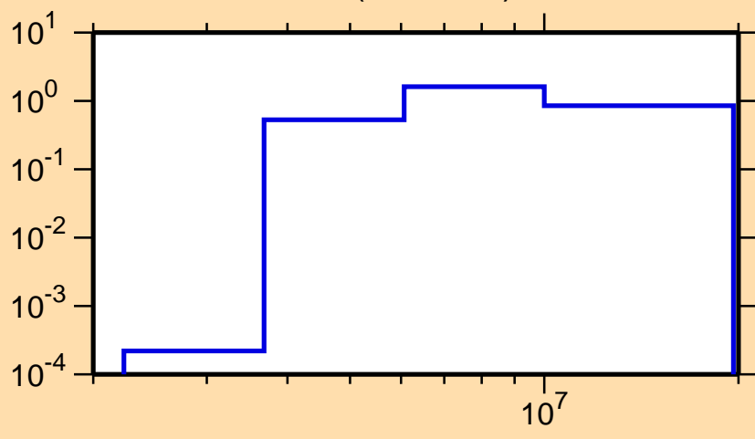
\sigma vs. E for ^{80}\text{Kr}(n,n\text{cont.})
