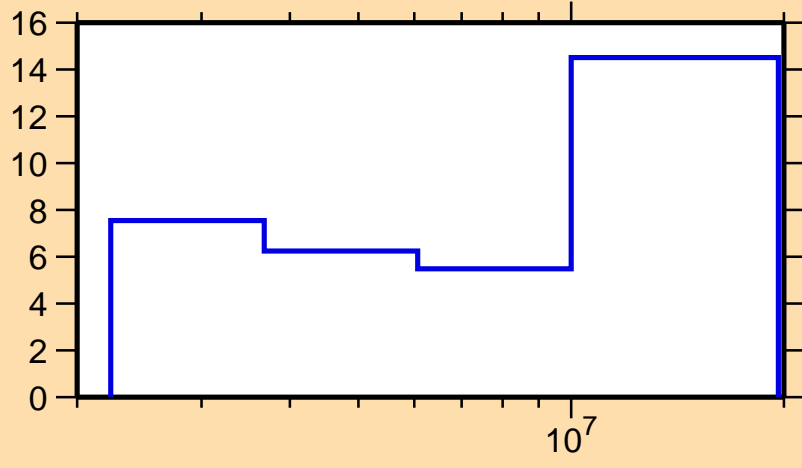
\Delta\sigma/\sigma vs. E for ^{80}\text{Kr}(n,inel.)
