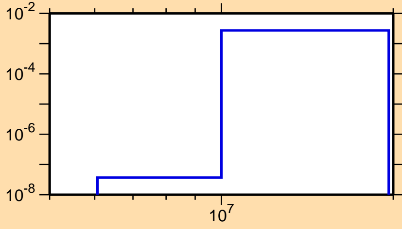
\sigma vs. E for ^{80}\text{Kr}(n,\alpha)
