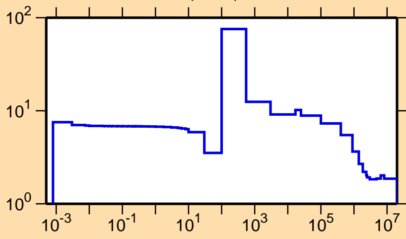
\sigma vs. E for ^{80}\text{Kr}(n,\text{el.})
