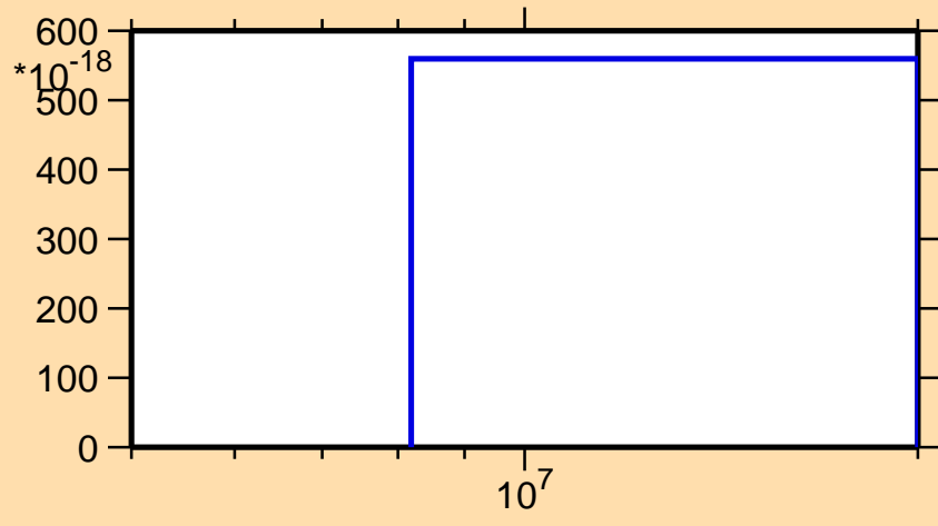
\sigma vs. E for ^{80}\text{Kr}(n,2n\alpha)
