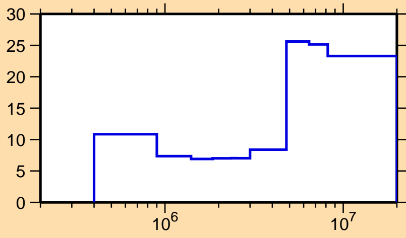
\Delta\sigma/\sigma vs. E for ^{80}\text{Kr}(n,n_1)
