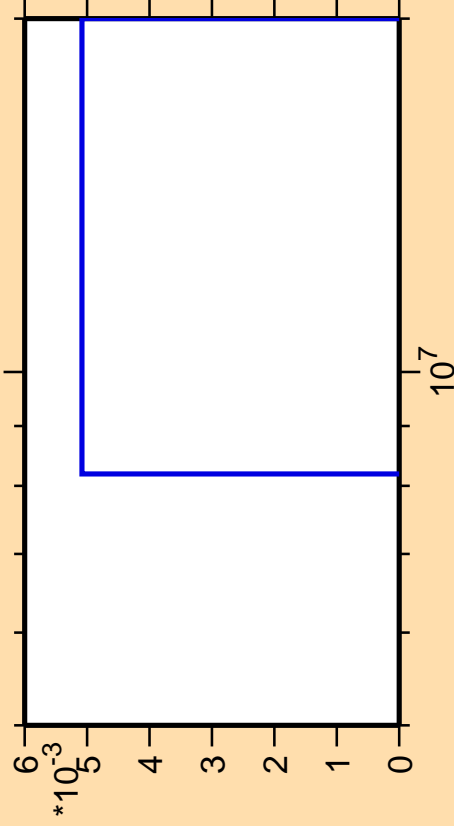
\Delta\sigma/\sigma vs. E for ^{80}\text{Kr}(\text{mt117})
