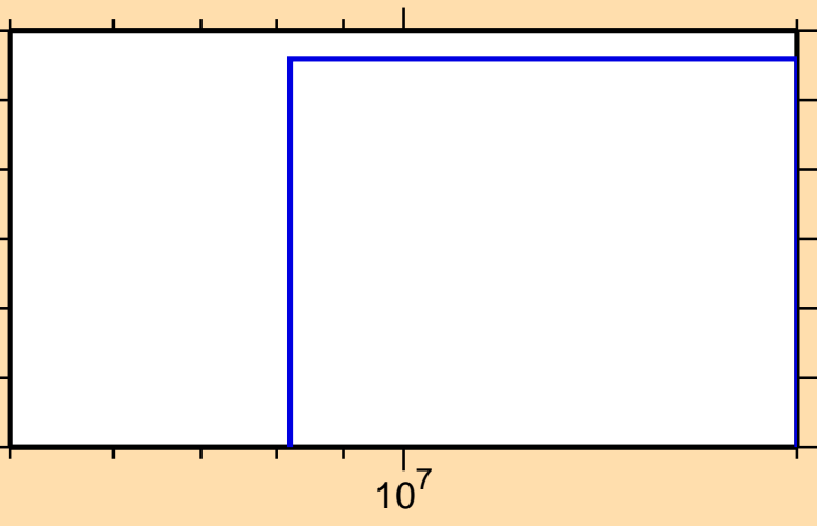
\sigma vs. E for ^{80}\text{Kr}(n,2n\alpha)
