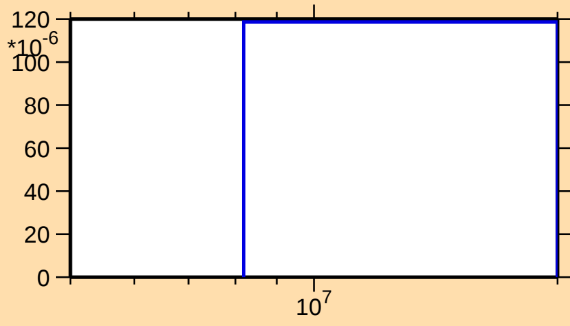
\sigma vs. E for ^{81}\text{Kr}(n,t)
