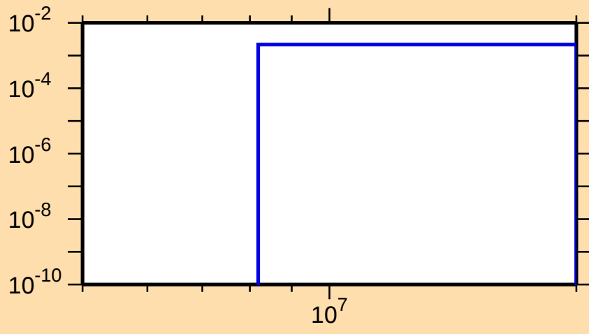
\sigma vs. E for ^{81}\text{Kr}(n,d)
