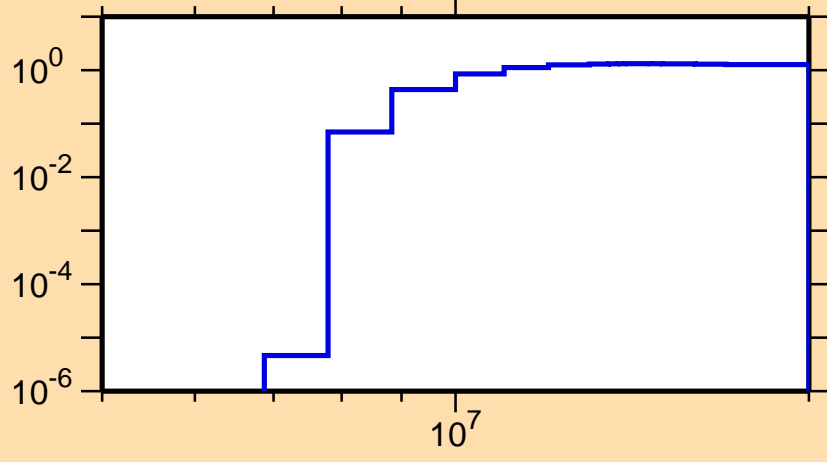
\sigma vs. E for ^{81}\text{Kr}(n,2n)
