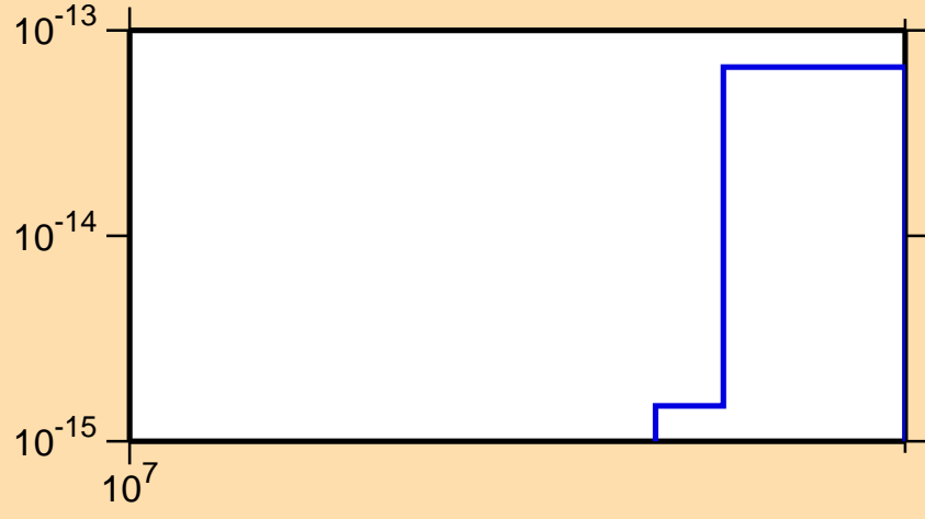
\sigma vs. E for ^{81}\text{Kr} (mt 34)
