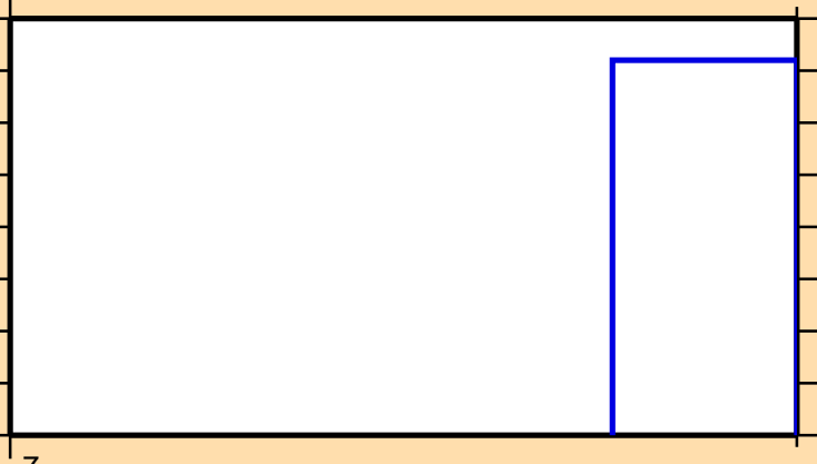
\sigma vs. E for ^{81}\text{Kr}(n,3n)
