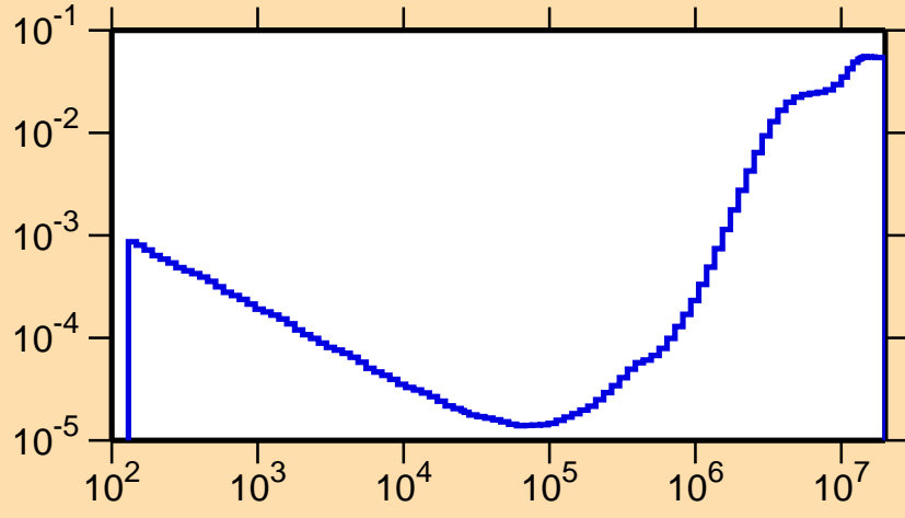
\sigma vs. E for ^{81}\text{Kr}(n,p)
