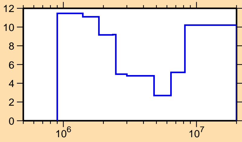
\Delta\sigma/\sigma vs. E for ^{81}\text{Kr}(n,tot.)
