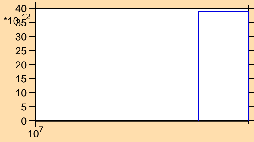
\sigma vs. E for ^{82}\text{Kr}(n,\text{nd})
