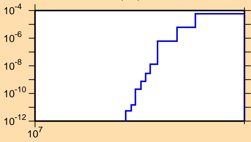
\sigma vs. E for ^{82}\text{Kr}(n,t)
