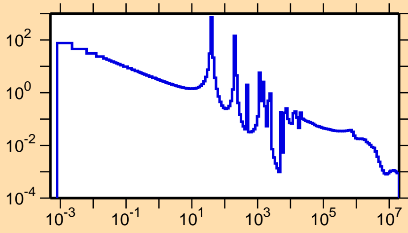
\sigma vs. E for ^{82}\text{Kr}(n,\gamma)
