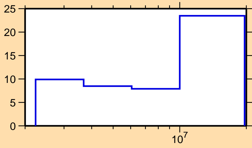
\Delta\sigma/\sigma vs. E for ^{82}\text{Kr}(n,ncont.)
