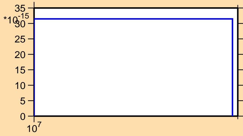
\sigma vs. E for ^{82}\text{Kr}(n,pd)
