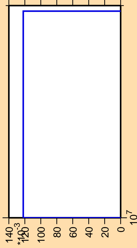
\Delta\sigma/\sigma vs. E for ^{82}\text{Kr}(n,pd)
