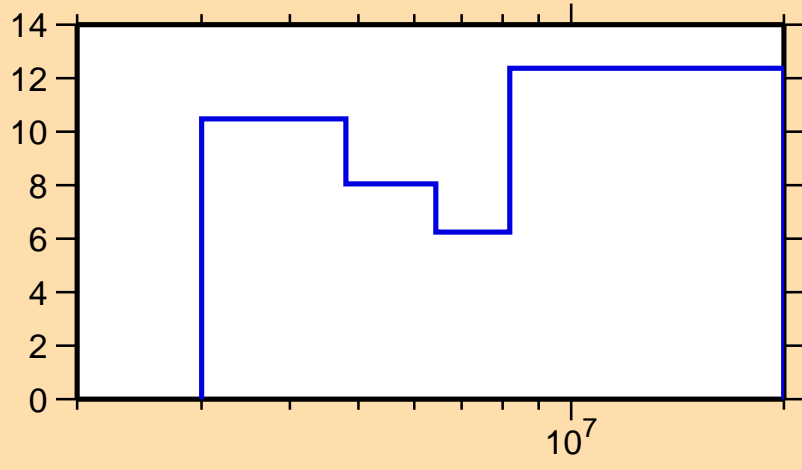
\Delta\sigma/\sigma vs. E for ^{82}\text{Kr}(n,el.)
