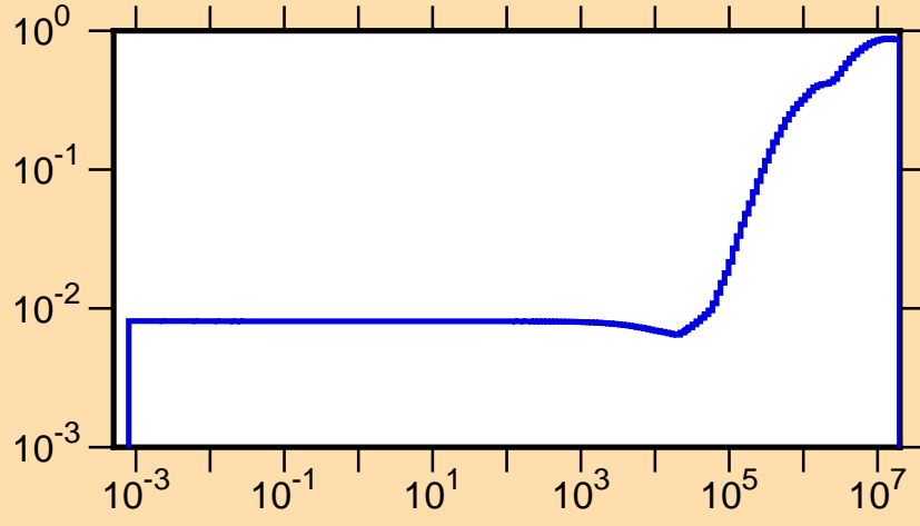
\mu vs. E for ^{83}\text{Kr}(\text{mt251})
