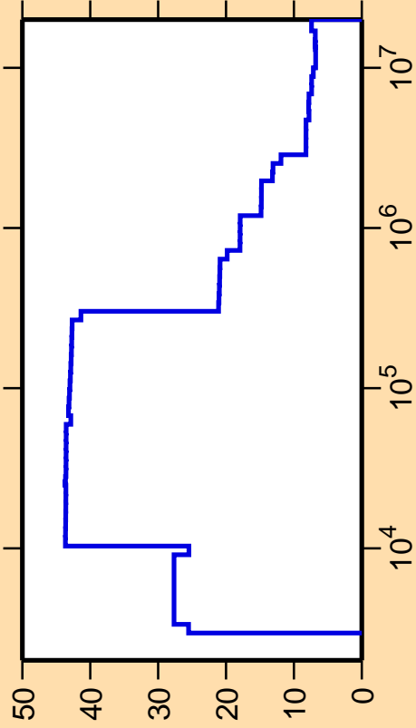
\Delta\sigma/\sigma vs. E for ^{83}\text{Kr}(n,\text{nonel.})
