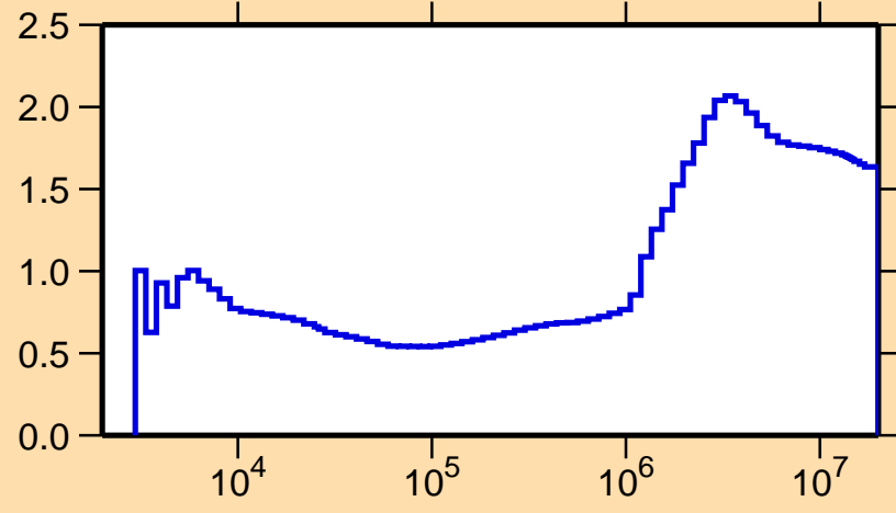
\sigma vs. E for ^{83}\text{Kr}(n,\text{nonel.})
