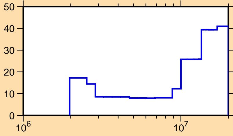
\Delta\sigma/\sigma vs. E for ^{83}\text{Kr}(n,n\text{cont.})
