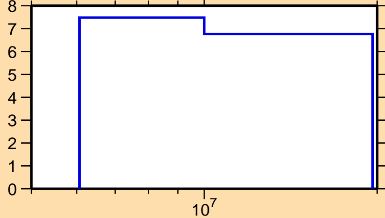
\Delta\sigma/\sigma vs. E for ^{83}\text{Kr}(n,\text{nonel.})
