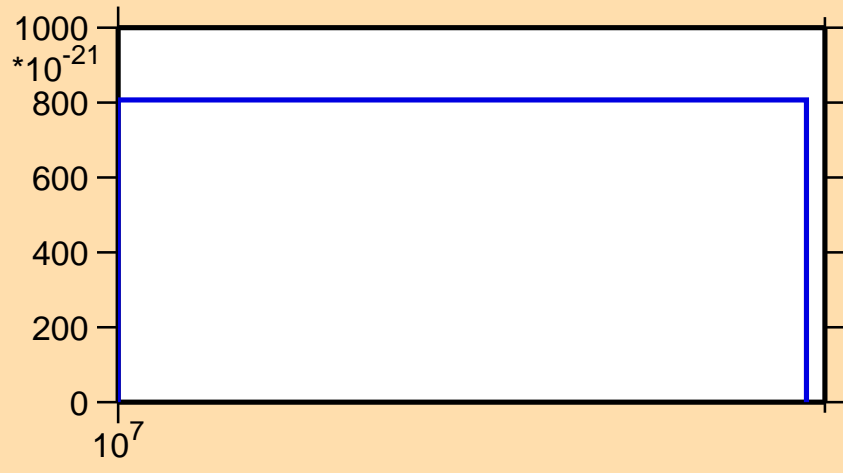
\sigma vs. E for ^{83}\text{Kr}(n,\text{pd})
