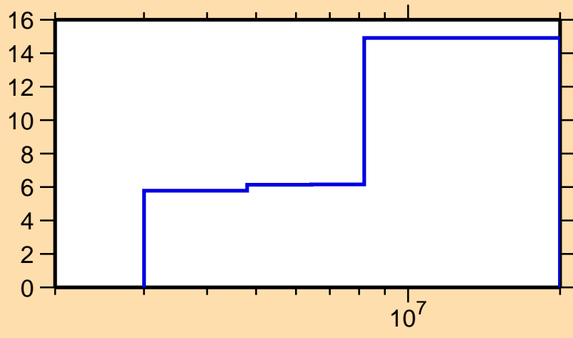
\Delta\sigma/\sigma vs. E for ^{84}\text{Kr}(n,inel.)
