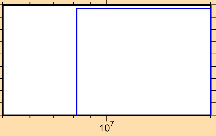
\sigma vs. E for ^{84}\text{Kr}(n,3n)
