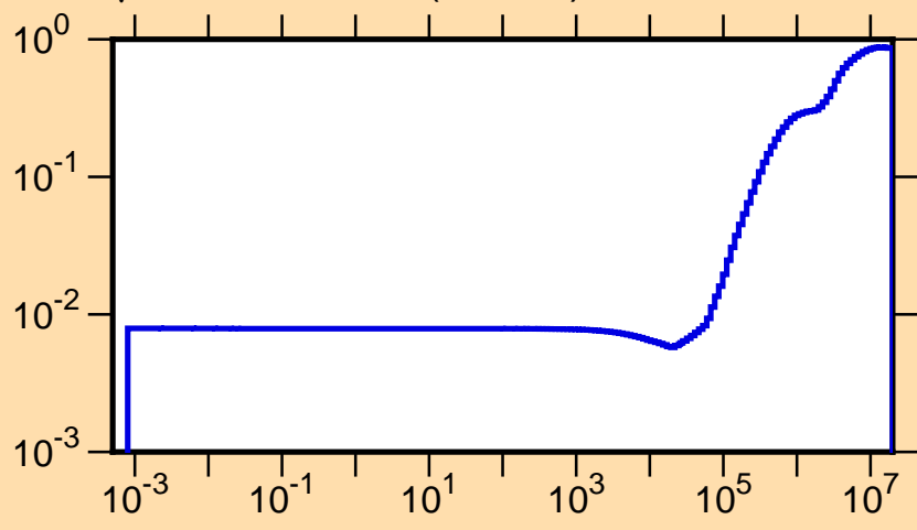
\mu vs. E for ^{85}\text{Kr}(\text{mt251})
