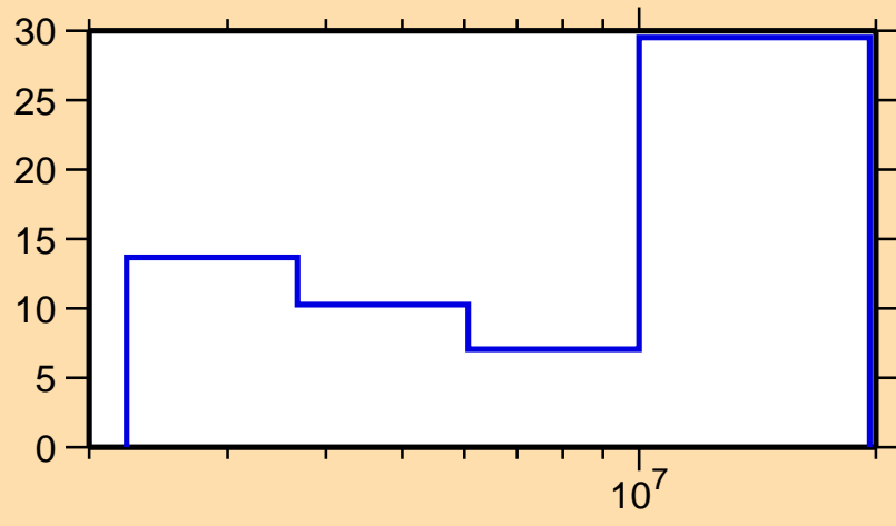
\Delta\sigma/\sigma vs. E for ^{85}\text{Kr}(n,n\text{cont.})
