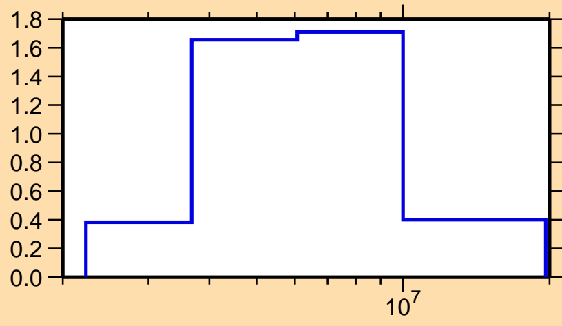
\sigma vs. E for ^{85}\text{Kr}(n,n\text{cont.})
