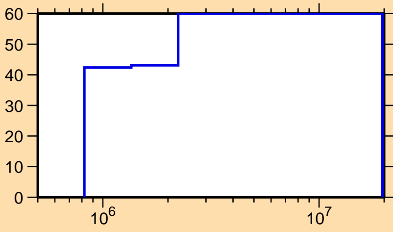
\Delta\sigma/\sigma vs. E for ^{85}\text{Kr}(n,\gamma)
