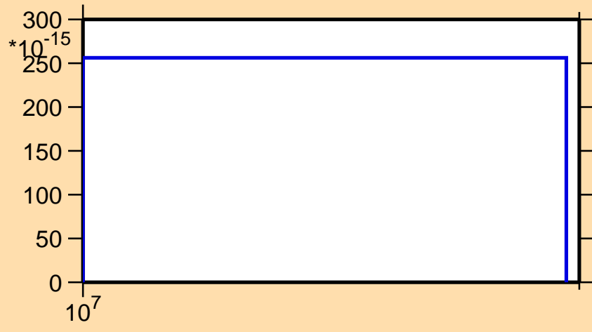
\sigma vs. E for ^{85}\text{Kr}(n,2np)
