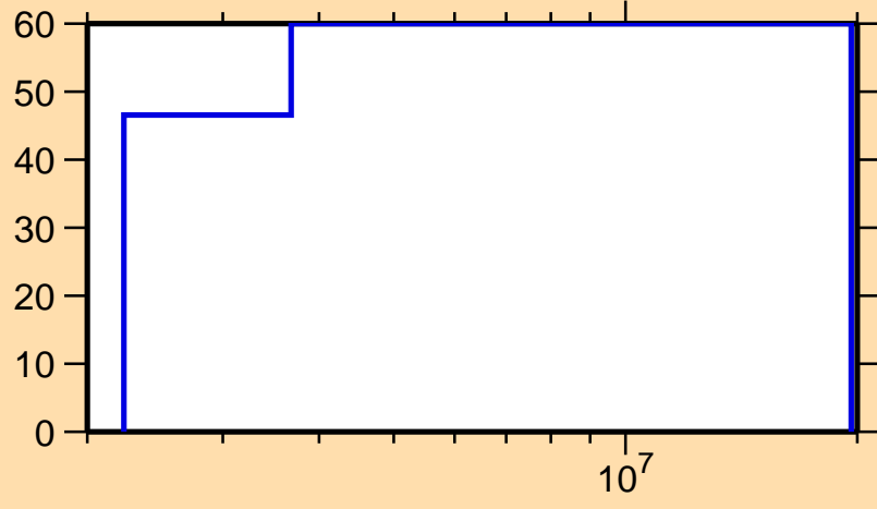
\Delta\sigma/\sigma vs. E for ^{85}\text{Kr}(n,n_1)
