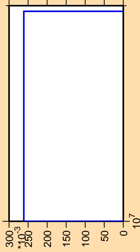
\Delta\sigma/\sigma vs. E for ^{85}\text{Kr}(n,2np)
