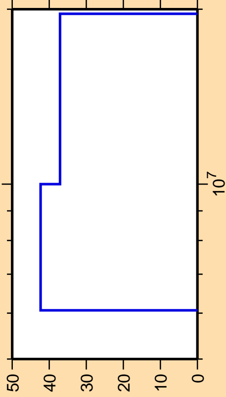
\Delta\sigma/\sigma vs. E for ^{85}\text{Kr}(n,p)
