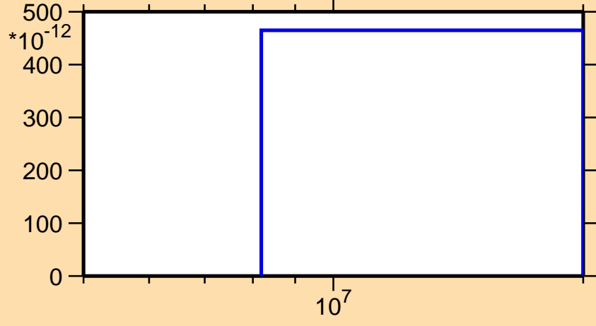
\sigma vs. E for ^{85}\text{Kr}(n,nd)
