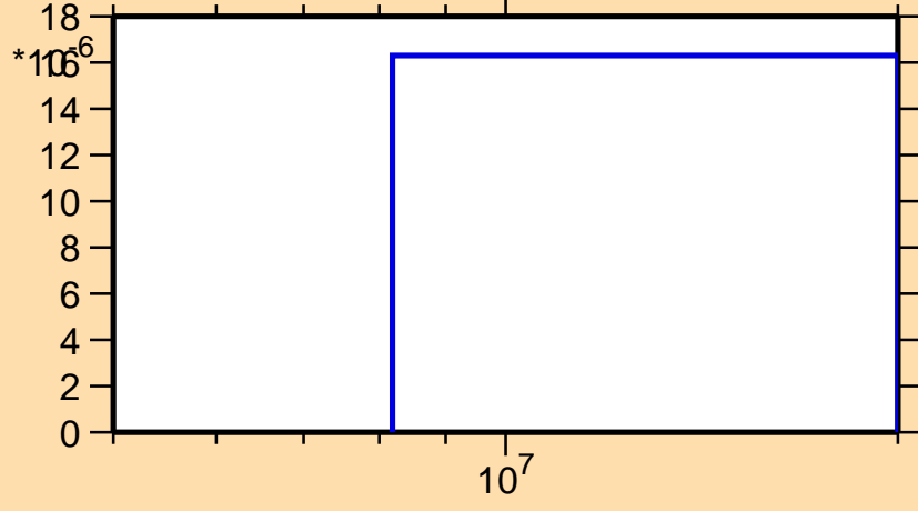
\sigma vs. E for ^{85}\text{Kr}(n,3n)
