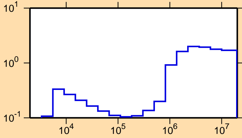
\sigma vs. E for ^{85}\text{Kr}(n,\text{nonel.})
