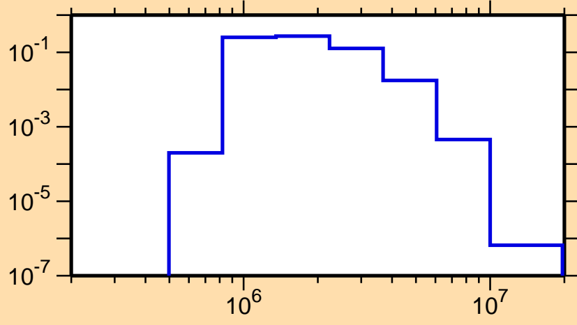
\sigma vs. E for ^{85}\text{Kr}(n,n_2)
