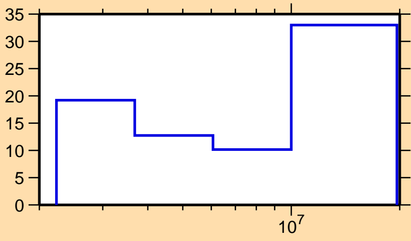
\Delta\sigma/\sigma vs. E for ^{85}\text{Kr}(n,ncont.)
