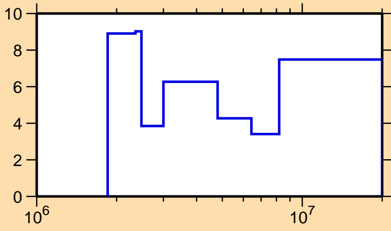
\Delta\sigma/\sigma vs. E for ^{85}\text{Kr}(n,tot.)
