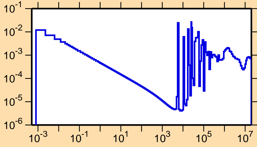
\sigma vs. E for ^{86}\text{Kr}(n,\gamma)
