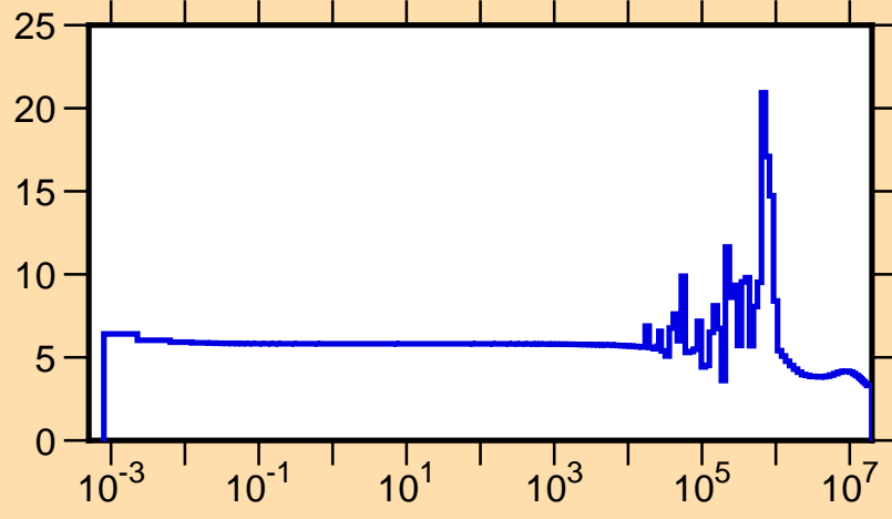
\sigma vs. E for ^{86}\text{Kr}(n,\text{tot.})
