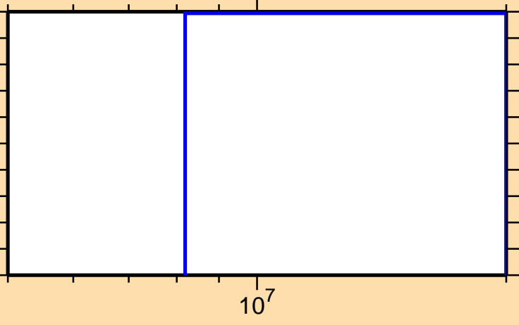
\sigma vs. E for ^{86}\text{Kr}(n,np)
