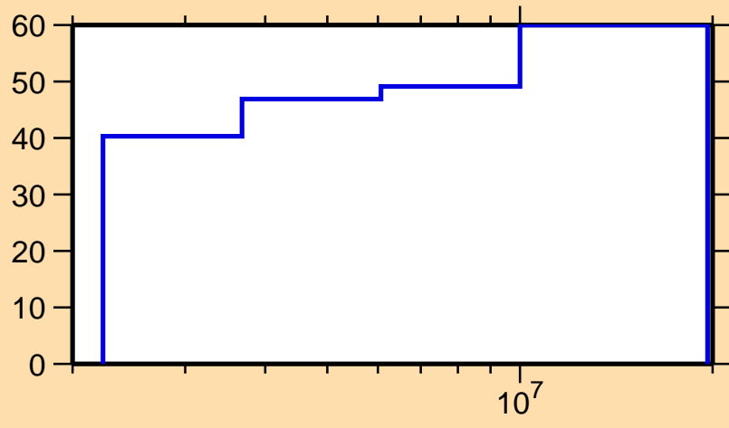
\Delta\sigma/\sigma vs. E for ^{87}\text{Kr}(n,\gamma)
