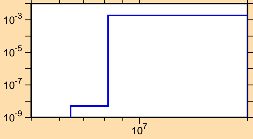
\sigma vs. E for ^{87}\text{Kr}(n,p)
