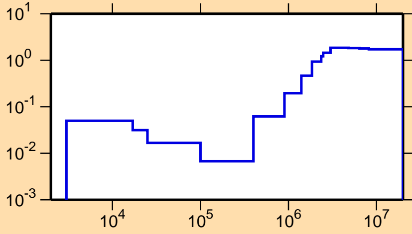
\sigma vs. E for ^{87}\text{Kr}(n,\text{nonel.})
