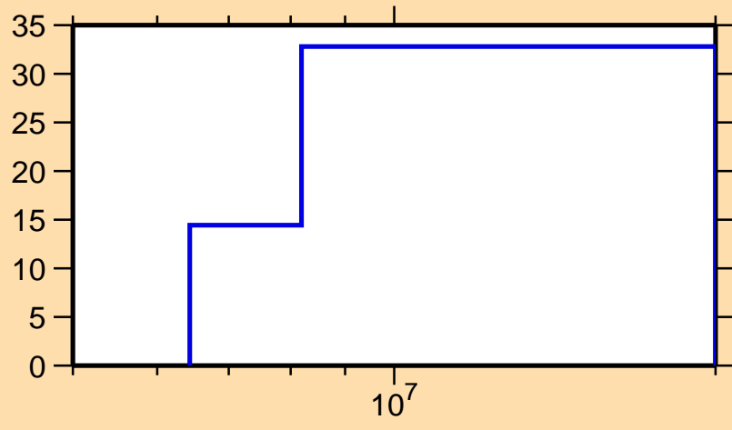
\Delta\sigma/\sigma vs. E for ^{87}\text{Kr}(n,ncont.)
