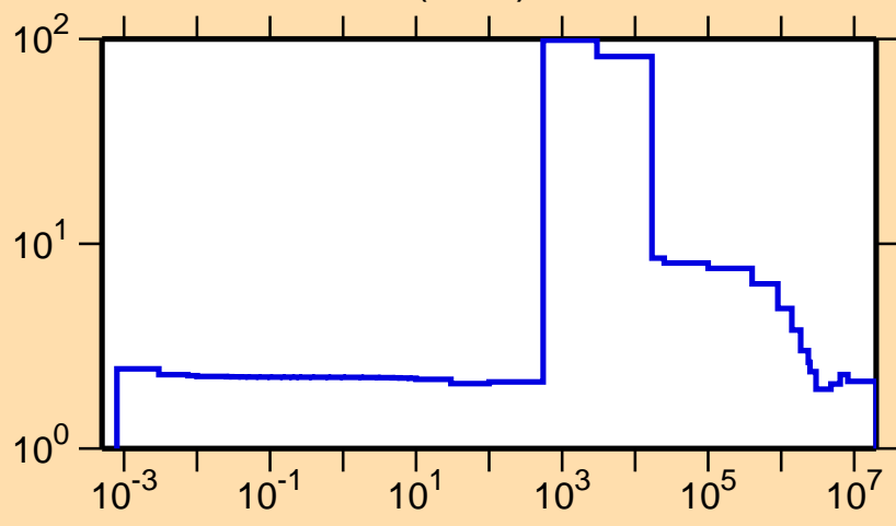
\sigma vs. E for ^{87}\text{Kr}(n,\text{el.})
