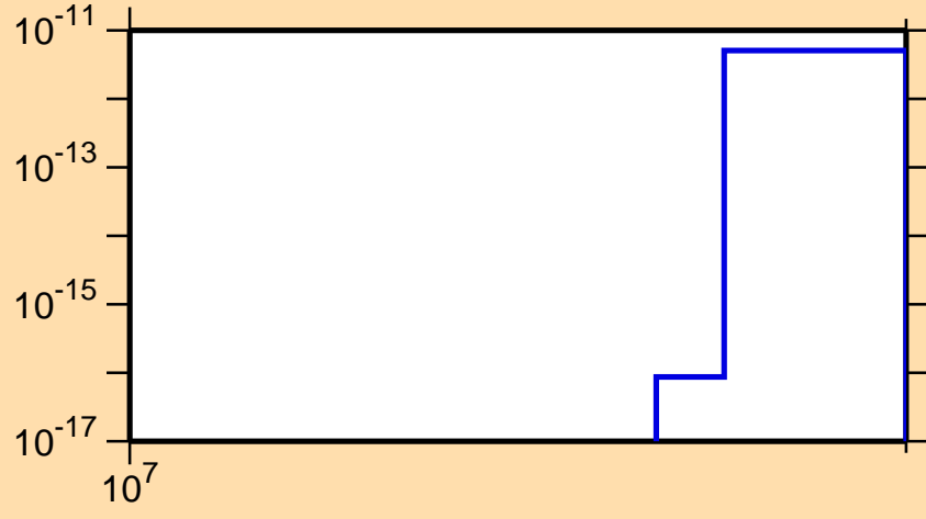
\sigma vs. E for ^{88}\text{Kr}(n,2n\alpha)
