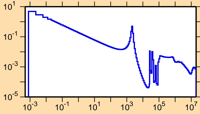
\sigma vs. E for ^{88}\text{Kr}(n,\gamma)
