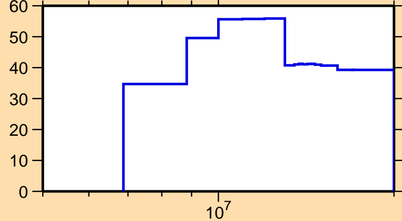
\Delta\sigma/\sigma vs. E for ^{88}\text{Kr}(n,\text{inel.})
