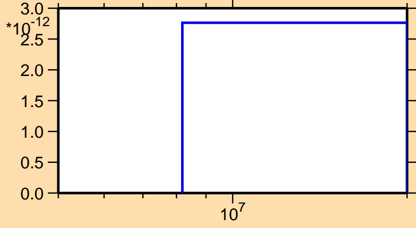
\sigma vs. E for ^{88}\text{Kr}(n,nd)
