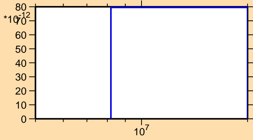
\sigma vs. E for ^{88}\text{Kr}(n,nt)
