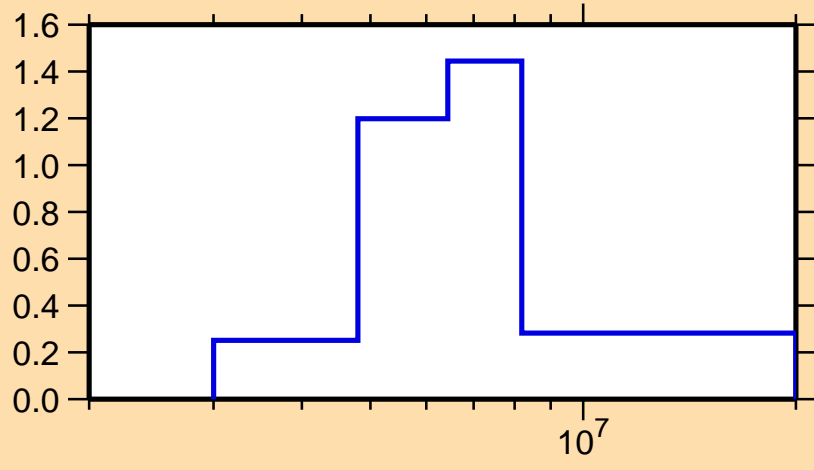
\sigma vs. E for ^{88}\text{Kr}(n,n\text{cont.})
