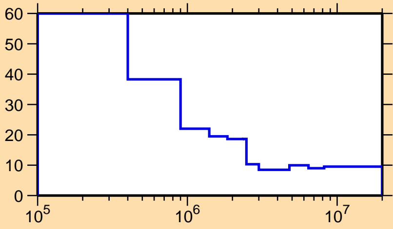
\Delta\sigma/\sigma vs. E for ^{88}\text{Kr}(n,\text{nonel.})
