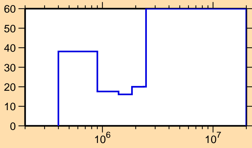
\Delta\sigma/\sigma vs. E for ^{88}\text{Kr}(n,n_1)
