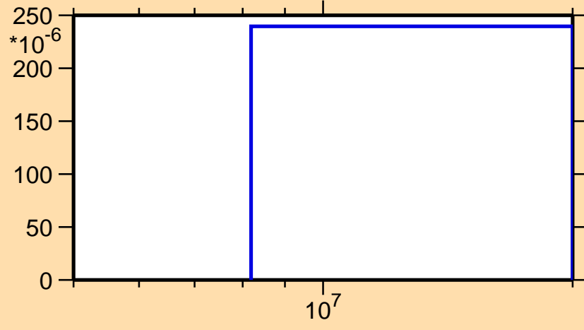
\sigma vs. E for ^{88}\text{Kr}(n,p)
