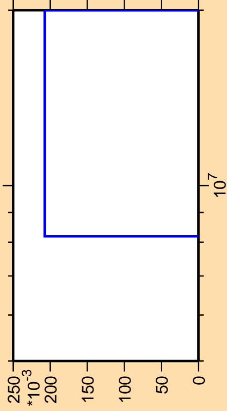
\Delta\sigma/\sigma vs. E for ^{88}\text{Kr}(n,2n\alpha)
