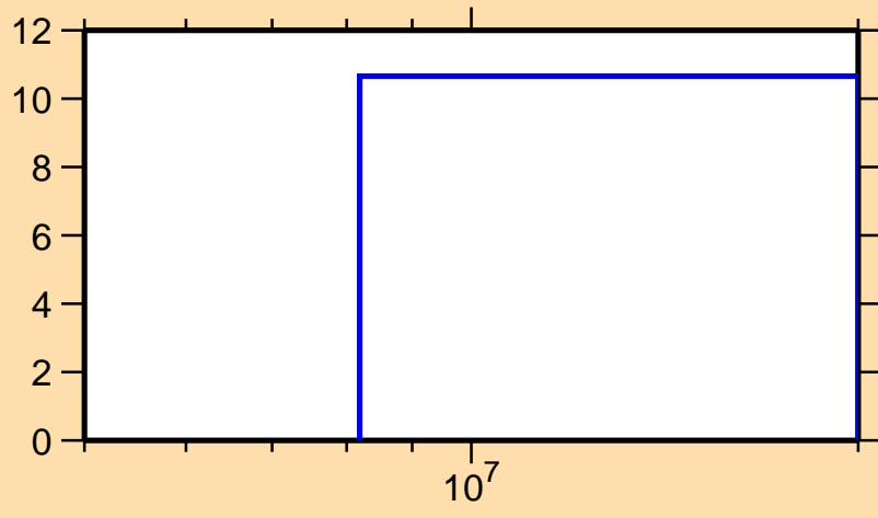
\Delta\sigma/\sigma vs. E for ^{88}\text{Kr}(n,2n)
