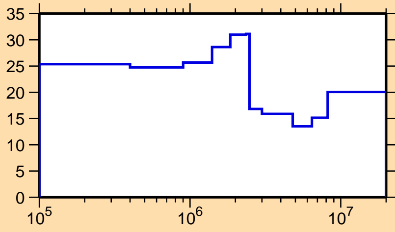
\Delta\sigma/\sigma vs. E for ^{88}\text{Kr}(n,\text{el.})
