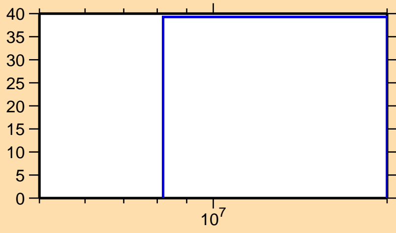
\Delta\sigma/\sigma vs. E for ^{88}\text{Kr}(n,p)
