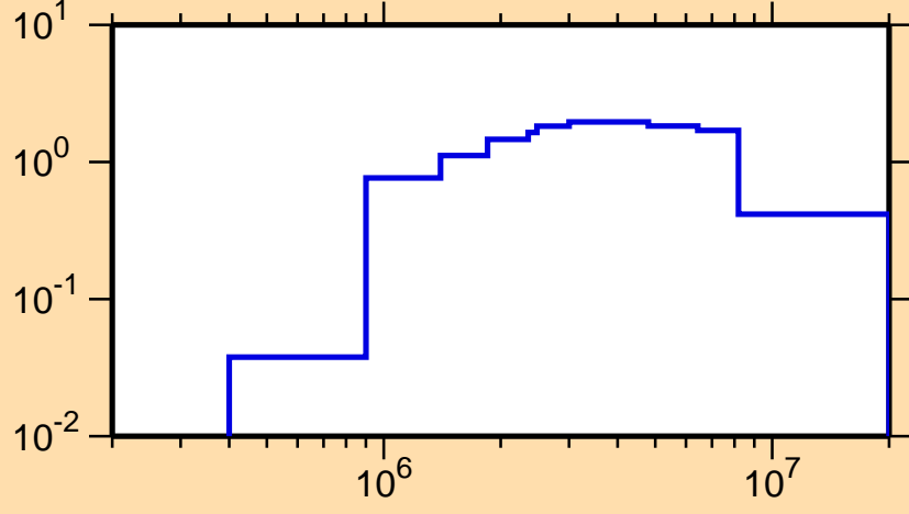
\sigma vs. E for ^{88}\text{Kr}(n,\text{inel.})
