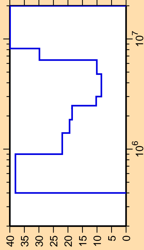
\Delta\sigma/\sigma vs. E for ^{88}\text{Kr}(n,\text{inel.})
