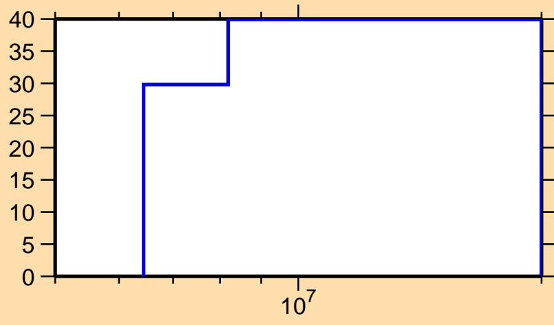
\Delta\sigma/\sigma vs. E for ^{88}\text{Kr}(n,\text{inel.})
