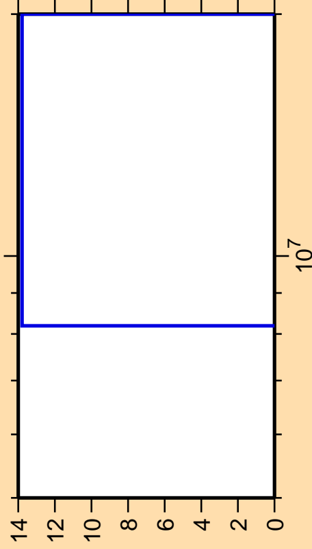
\Delta\sigma/\sigma vs. E for ^{88}\text{Kr}(n,nd)
