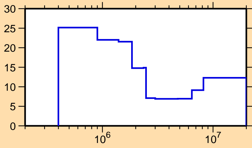
\Delta\sigma/\sigma vs. E for ^{88}\text{Kr}(n,\text{tot.})
