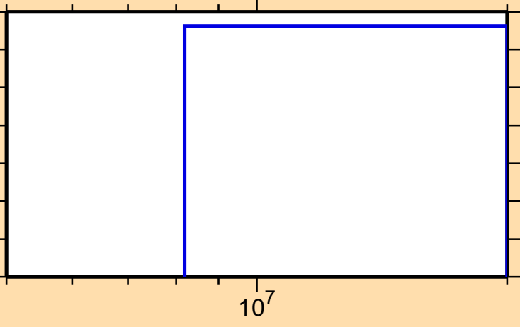
\sigma vs. E for ^{88}\text{Kr}(n,3n)
