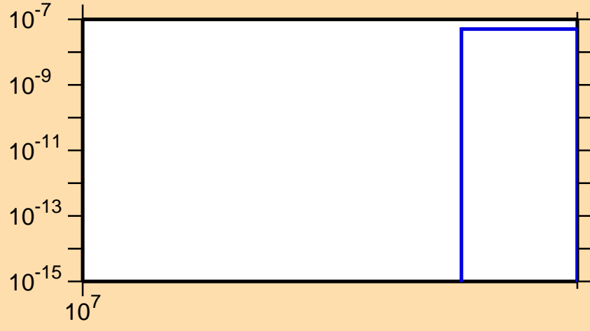
\sigma vs. E for ^{91}\text{Kr}(n,\text{nd})
