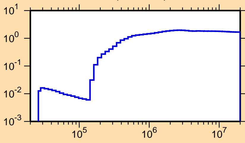
\sigma vs. E for ^{91}\text{Kr}(n,\text{nonel.})
