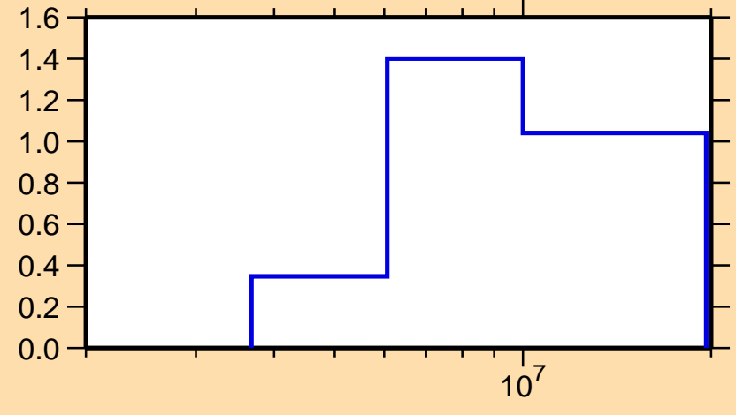
\sigma vs. E for ^{91}\text{Kr}(n,2n)
