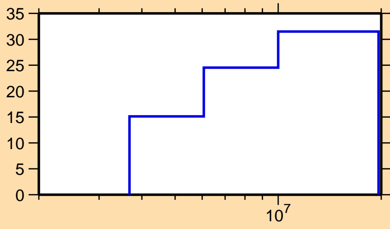
\Delta\sigma/\sigma vs. E for ^{91}\text{Kr}(n, el.)
