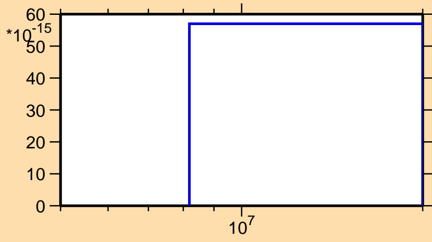
\sigma vs. E for ^{91}\text{Kr}(n,2np)
