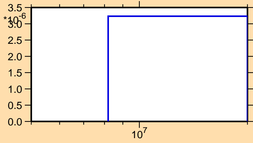
\sigma vs. E for ^{91}\text{Kr}(n,\alpha)
