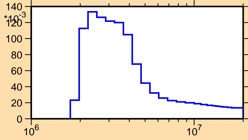
\sigma vs. E for ^{92}\text{Kr}(n,n_4)
