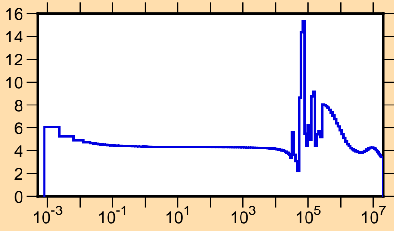
\sigma vs. E for ^{92}\text{Kr}(n,\text{tot.})
