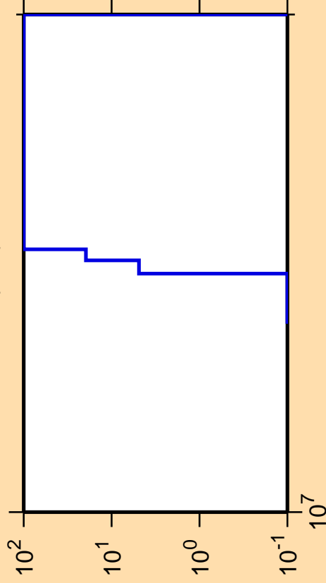
\Delta\sigma/\sigma vs. E for ^{92}\text{Kr}(n,d)
