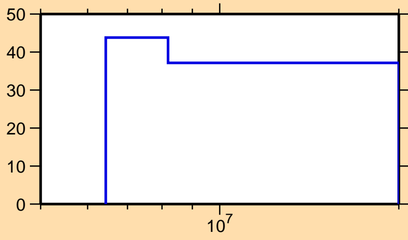
\Delta\sigma/\sigma vs. E for ^{92}\text{Kr}(n,n\text{cont.})
