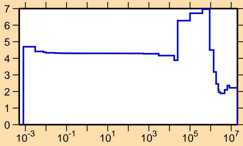
\sigma vs. E for ^{92}\text{Kr}(n,\text{el.})
