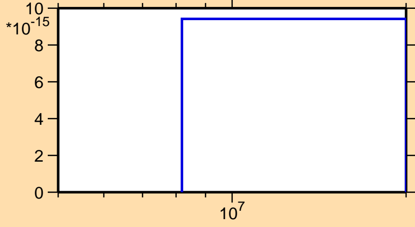
\sigma vs. E for ^{92}\text{Kr}(n,nd)
