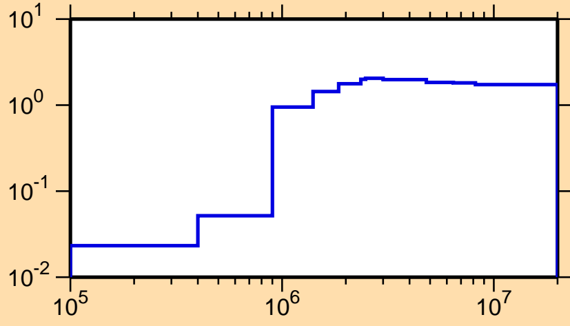
\sigma vs. E for ^{92}\text{Kr}(n,\text{nonel.})
