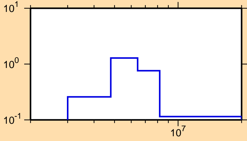
\sigma vs. E for ^{92}\text{Kr}(n,n\text{cont.})
