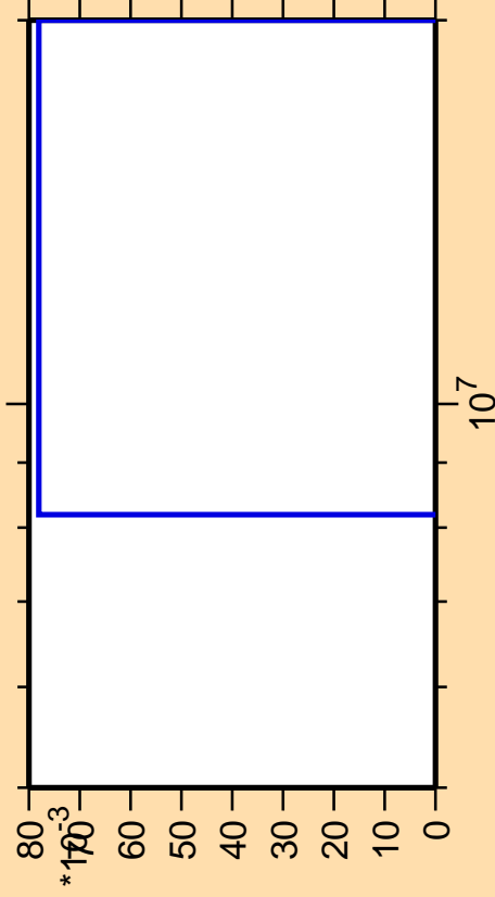
\Delta\sigma/\sigma vs. E for ^{92}\text{Kr}(n,nd)
