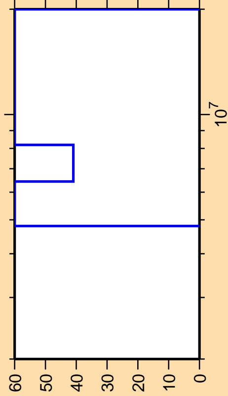
\Delta\sigma/\sigma vs. E for ^{92}\text{Kr}(n,2n)
