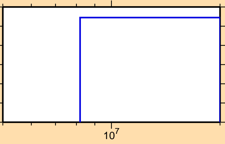
\sigma vs. E for ^{92}\text{Kr}(n,np)
