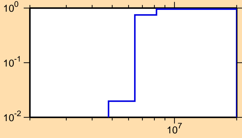
\sigma vs. E for ^{92}\text{Kr}(n,2n)
