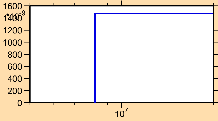
\sigma vs. E for ^{92}\text{Kr}(n,p)
