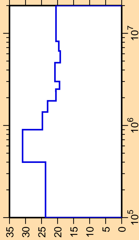
\Delta\sigma/\sigma vs. E for ^{92}\text{Kr}(n,\text{nonel.})
