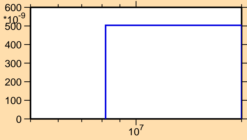
\sigma vs. E for ^{92}\text{Kr}(n,n\alpha)
