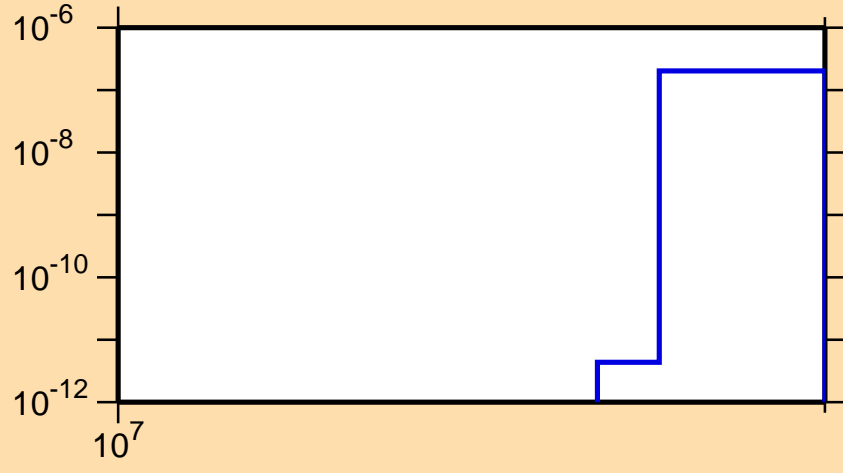
\sigma vs. E for ^{93}\text{Kr}(n,nt)
