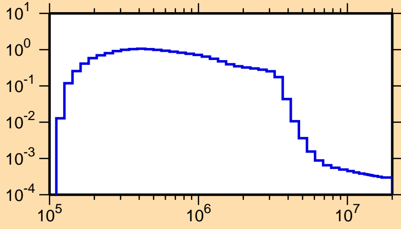
\sigma vs. E for ^{93}\text{Kr}(n,n_1)
