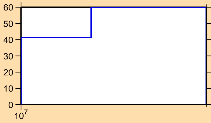
\Delta\sigma/\sigma vs. E for ^{93}\text{Kr}(n,el.)
