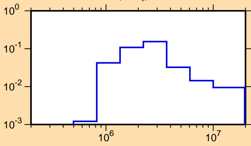
\sigma vs. E for ^{93}\text{Kr}(n,n_4)
