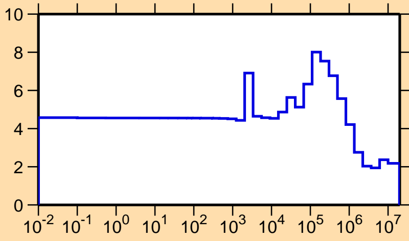
\sigma vs. E for ^{93}\text{Kr}(n,\text{el.})
