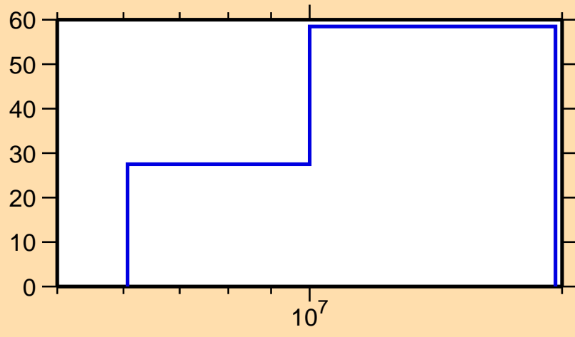
\Delta\sigma/\sigma vs. E for ^{93}\text{Kr}(n,n\text{cont.})
