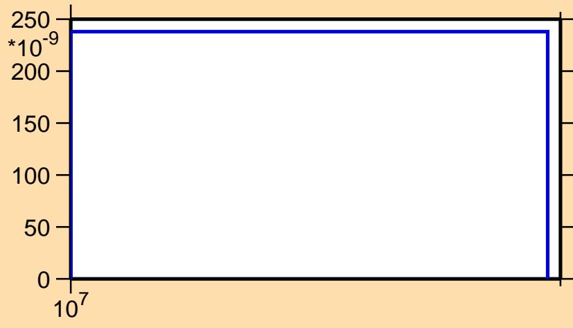
\sigma vs. E for ^{93}\text{Kr}(n,d)
