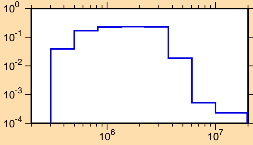
\sigma vs. E for ^{93}\text{Kr}(n,n_2)
