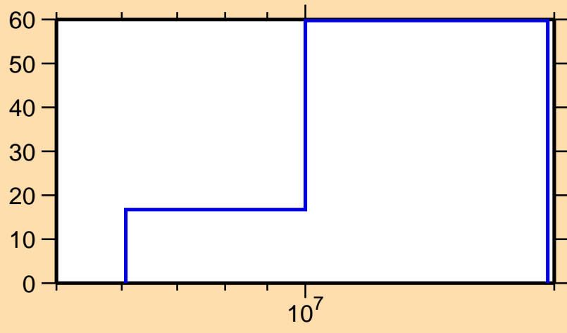
\Delta\sigma/\sigma vs. E for ^{93}\text{Kr}(n,\text{el.})
