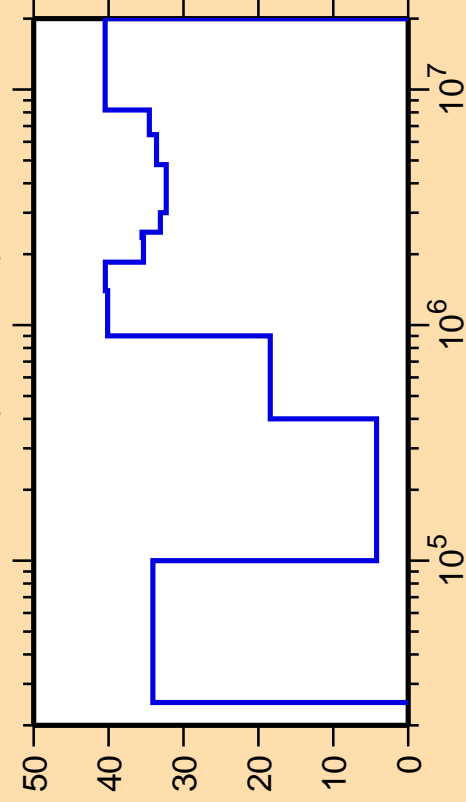
\Delta\sigma/\sigma vs. E for ^{93}\text{Kr}(n,\text{nonel.})
