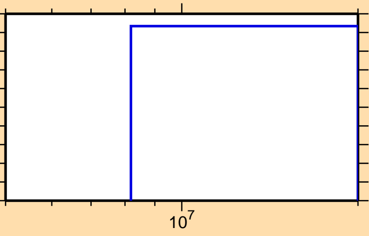
\sigma vs. E for ^{93}\text{Kr}(n,np)
