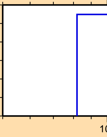
\sigma vs. E for ^{93}\text{Kr}(n,2np)
