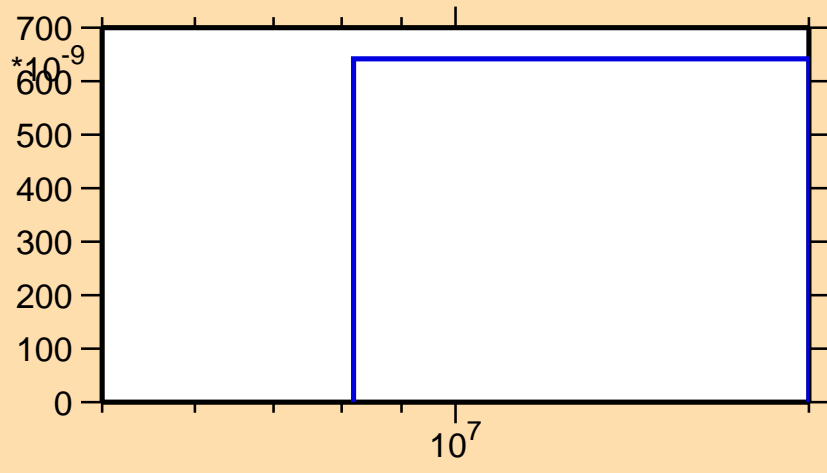
\sigma vs. E for ^{93}\text{Kr}(n,n\alpha)
