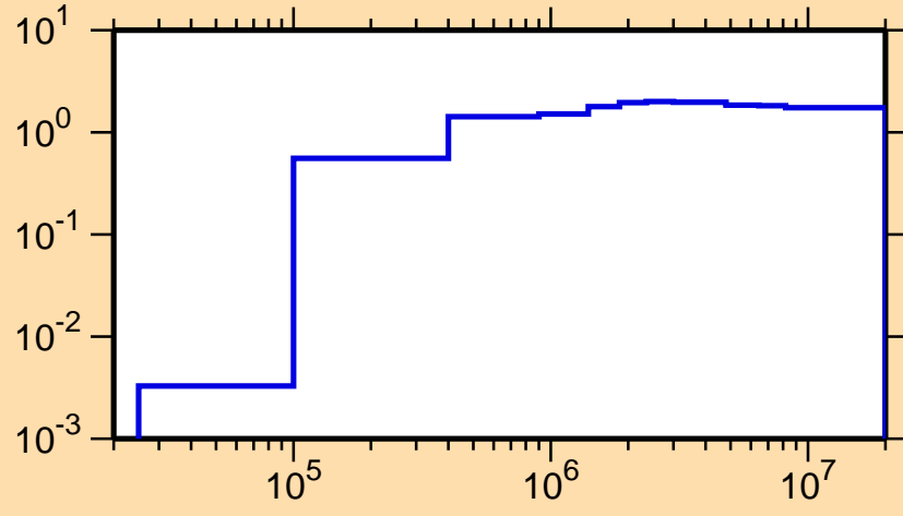
\sigma vs. E for ^{93}\text{Kr}(n,\text{nonel.})
