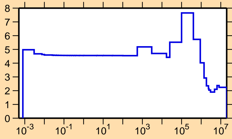
\sigma vs. E for ^{93}\text{Kr}(n,\text{el.})
