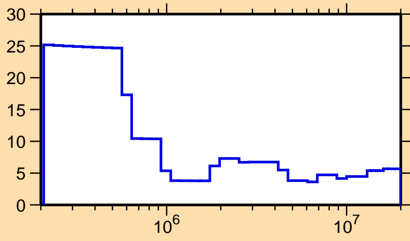
\Delta\sigma/\sigma vs. E for ^{119}\text{La}(n,\text{tot.})
