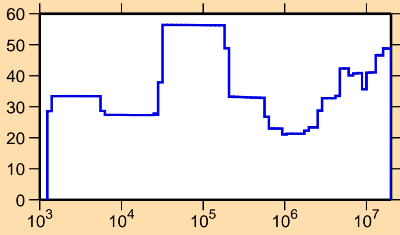
\Delta\sigma/\sigma vs. E for ^{119}\text{La}(n,p)
