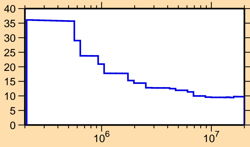
\Delta\sigma/\sigma vs. E for ^{119}\text{La}(n,\text{nonel.})
