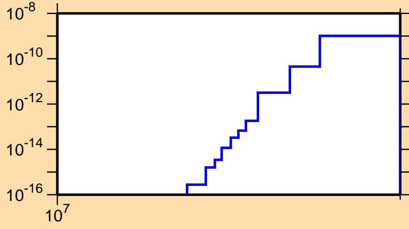
\sigma vs. E for ^{119}\text{La} (mt 34)
