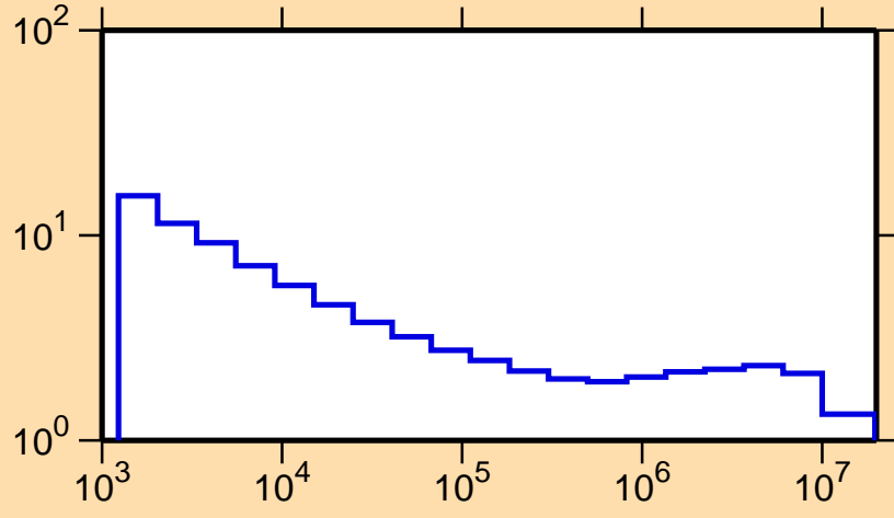
\sigma vs. E for ^{119}\text{La}(n,\text{nonel.})
