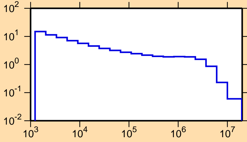
\sigma vs. E for ^{119}\text{La}(n,p)
