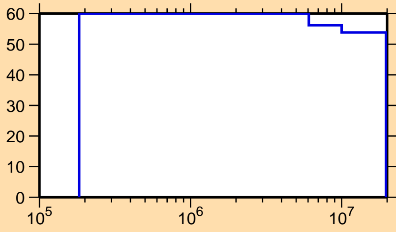
\Delta\sigma/\sigma vs. E for ^{119}\text{La}(n,n\text{cont.})
